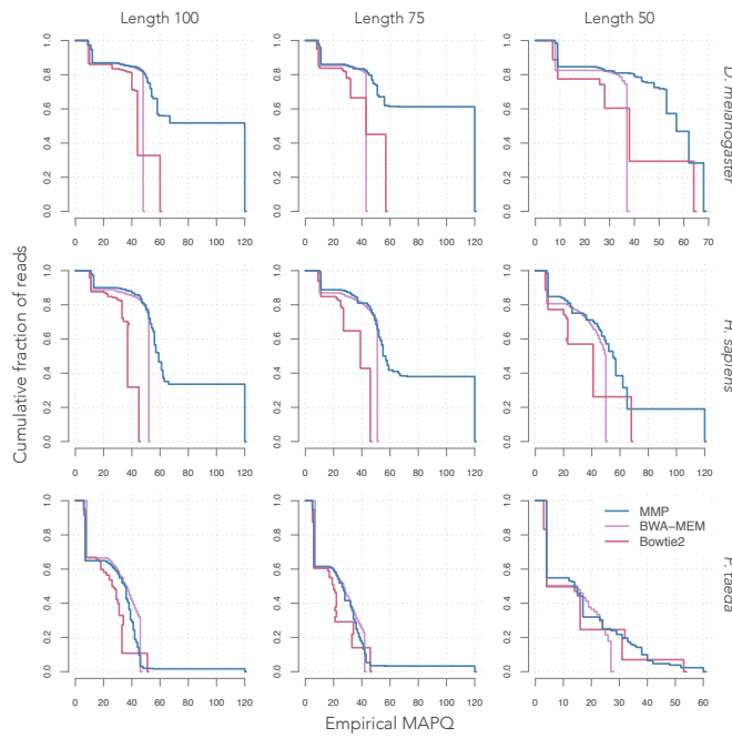
Supplementary Figure 2: Mapping accuracy with 2% error rate. The representations are as in Figure 7.
