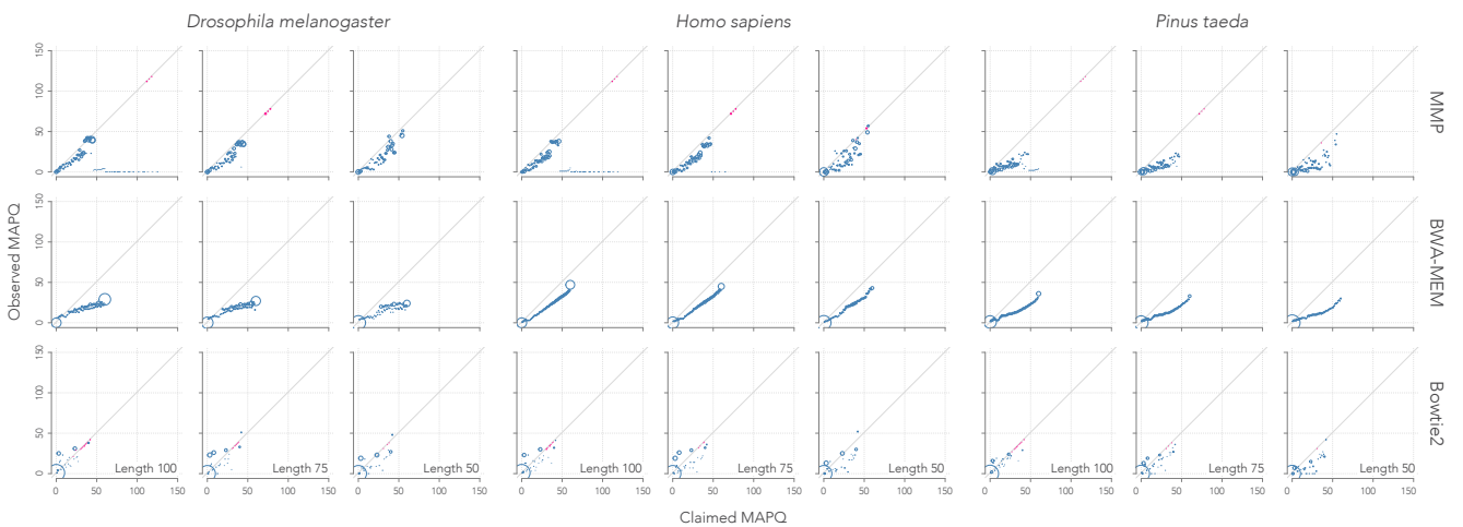
Supplementary Figure 7: Faithfulness with 10% error rate. The representations are the same as in Figure 6.
