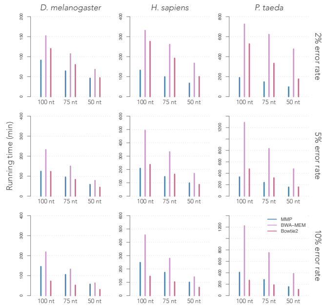
Supplementary Figure 1: Resource usage at 2, 5 and 10% error rate. The representations are as in Figure 8 (the memory footprint does not depend on the error rate of the sequencing process).
