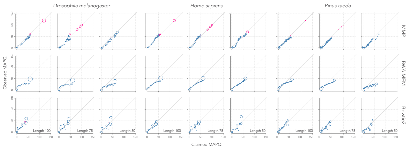
Supplementary Figure 5: Faithfulness with 2% error rate. The representations are the same as in Figure 6.
