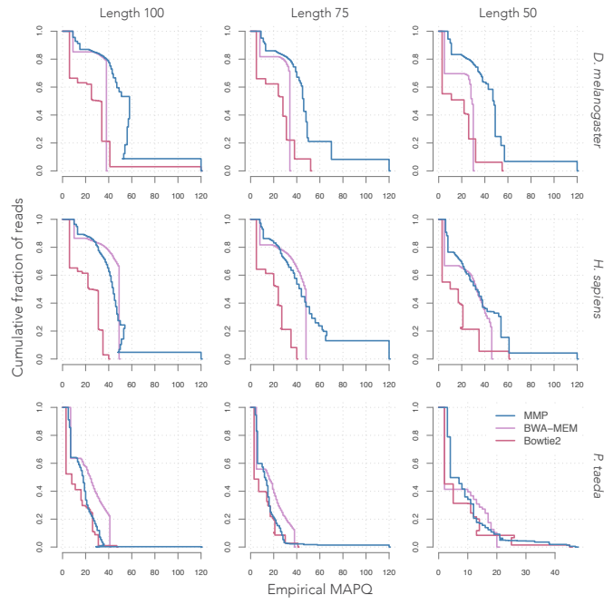
Supplementary Figure 3: Mapping accuracy with 5% error rate. The representations are as in Figure 7.
