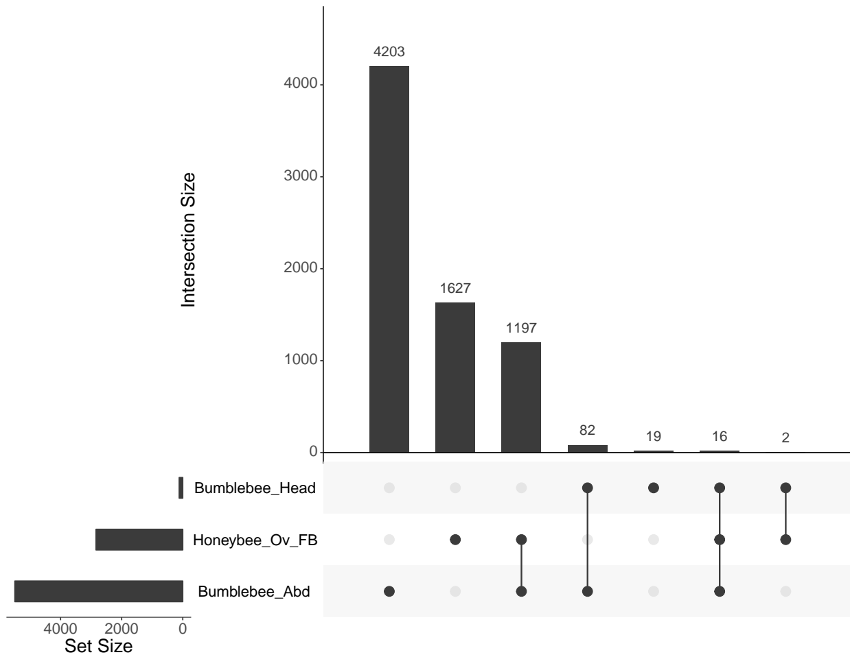
Figure S12: Overlapping genes showing differential expression between reproductive (queen-right) and sterile (queen-less) workers of B. terrestris head and abdomen tissue and A. mellifera ovary/fatbody tissue (genes identified in Galbraith et al. (2016)). The set size indicates the number of genes in each list. The intersection size shows how many genes the corresponding lists have in common. A single dot refers to the number of genes unique to each list.
