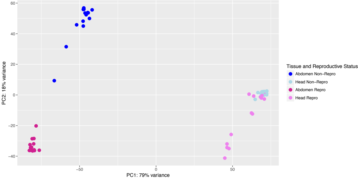
Figure S1: PCA plot based on gene expression data. Samples separate by tissue type along PC1 and by reproductive status along PC2.
