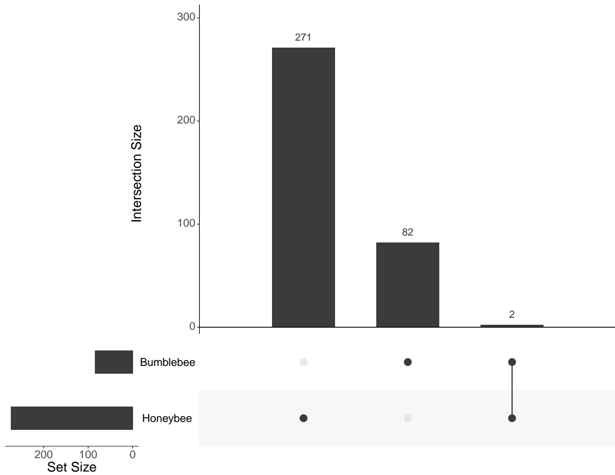
Figure S10: Overlapping genes showing parent-of-origin expression in reproductive (queen-right) and sterile (queen-less) workers of B. terrestris and A. mellifera (genes identified in Galbraith et al. (2016)). The set size indicates the number of genes in each list. The intersection size shows how many genes the corresponding lists have in common. A single dot refers to the number of genes unique to each list.
