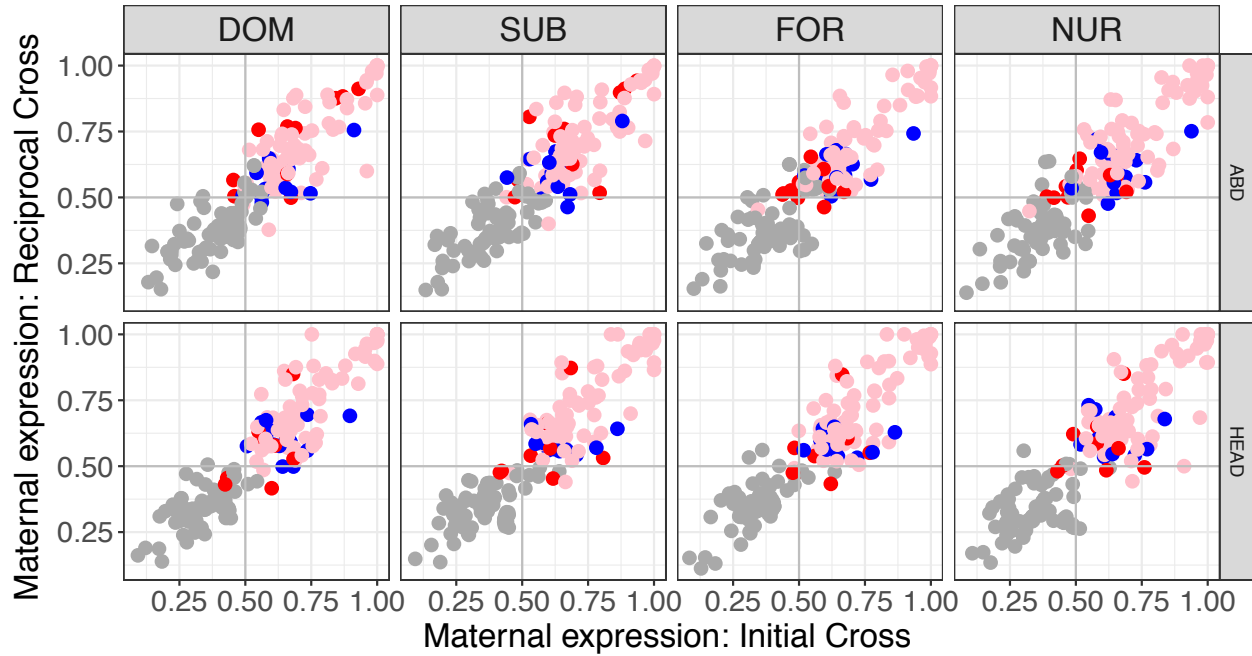
Figure S6: The proportion of maternal expression for each behavioural reproductive type per tissue type for all genes found to show significant parental expression bias. DOM represents dominant reproductives. SUB represents subordinate reproductives. FOR represents sterile foragers. NUR represents sterile nurses. ABD refers to abdominal tissue and HEAD refers to head tissue. Each dot represents a gene, the pink dots highlight significantly maternally expressed genes in both sterile and reproductive workers. The red dots are genes showing significant maternal expression bias in reproductive workers only and the blue dots show significant maternal expression bias in sterile workers only.
