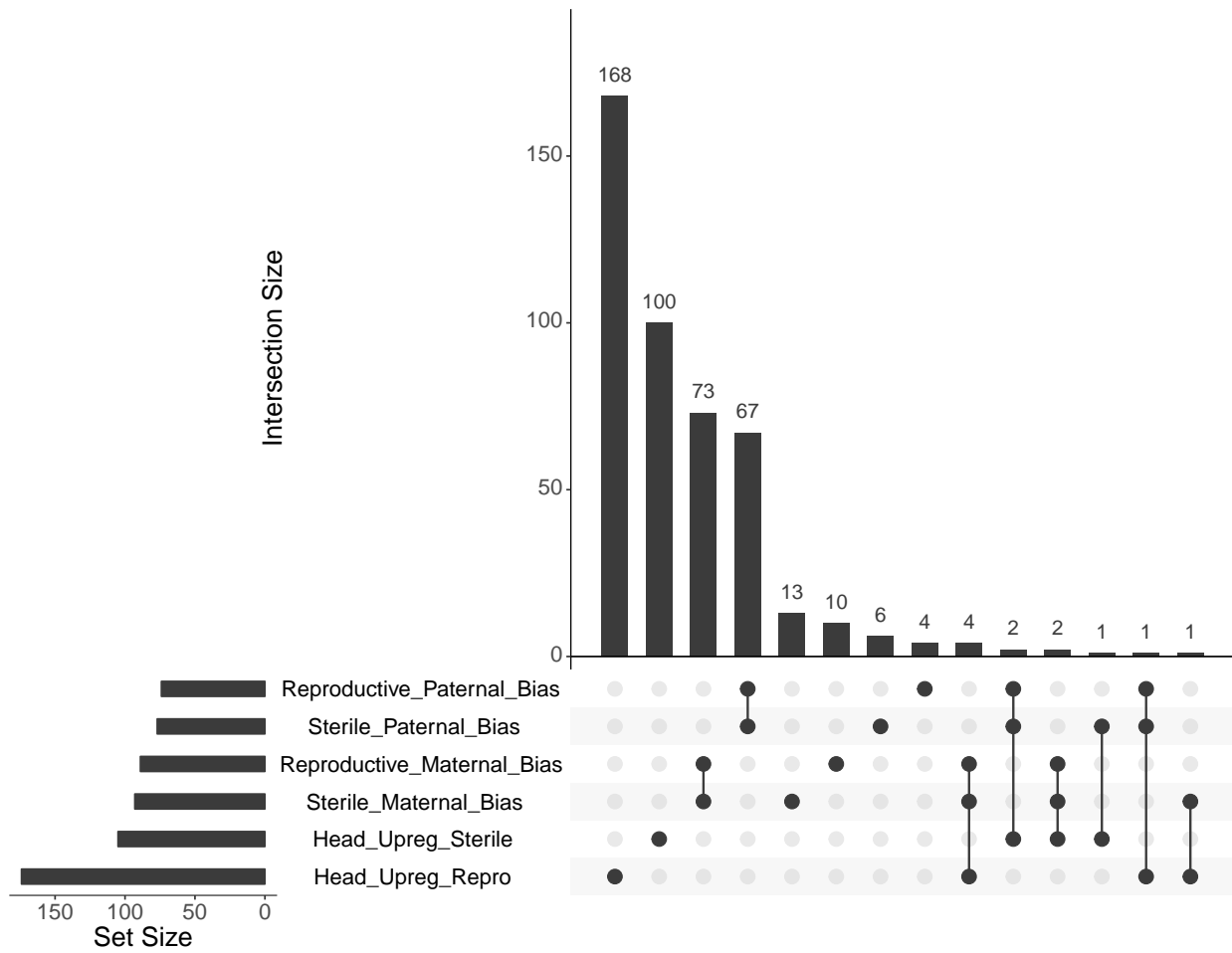
Figure S8: Overlapping genes showing parent-of-origin expression in reproductive (queen-right) and sterile (queen-less) workers with genes showing differential expression in head tissue. The set size indicates the number of genes in each list. The intersection size shows how many genes the corresponding lists have in common. A single dot refers to the number of genes unique to each list. 7/103 genes showing maternal bias are also differentially expressed in the head.
