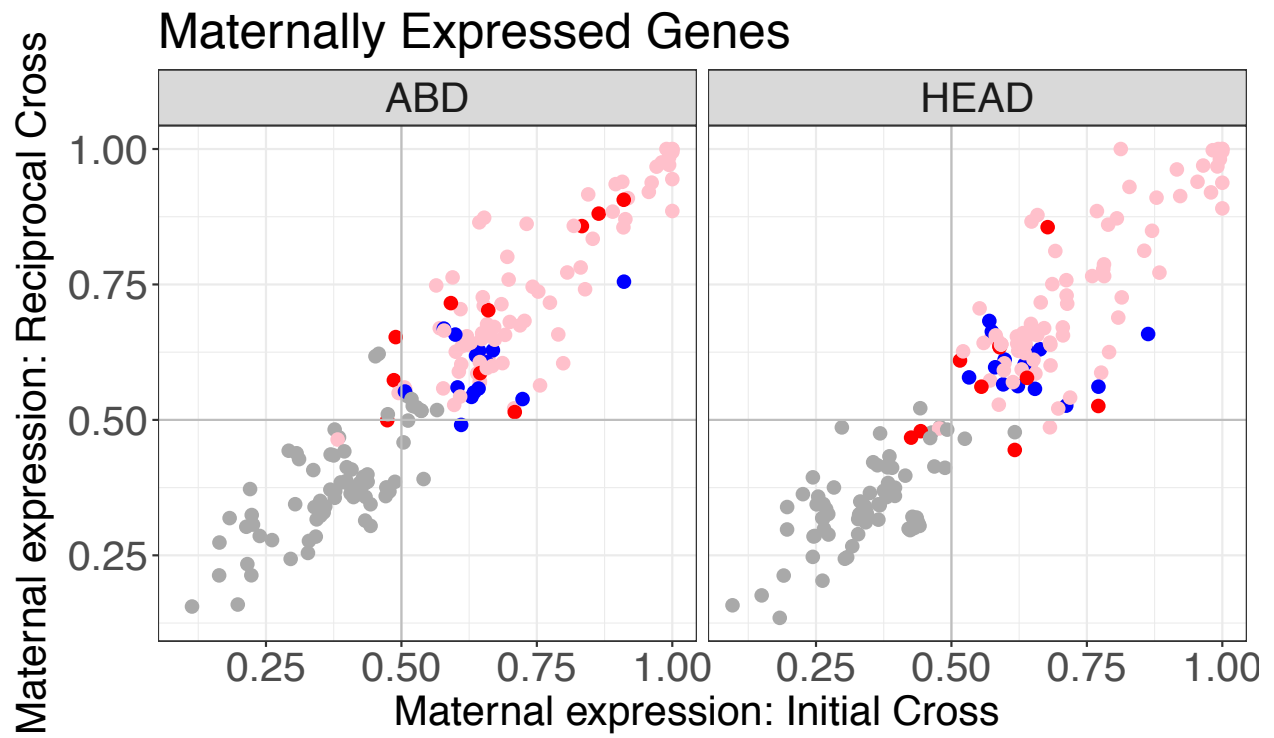
Figure S2: The proportion of maternal expression for each tissue type of all genes found to show significant parental expression bias. ABD refers to abdominal tissue and HEAD refers to head tissue. Each dot represents a gene, the pink dots highlight significantly maternally expressed genes in both sterile and reproductive workers. The red dots are genes showing significant maternal expression bias in reproductive workers only and the blue dots show significant maternal expression bias in sterile workers only.
