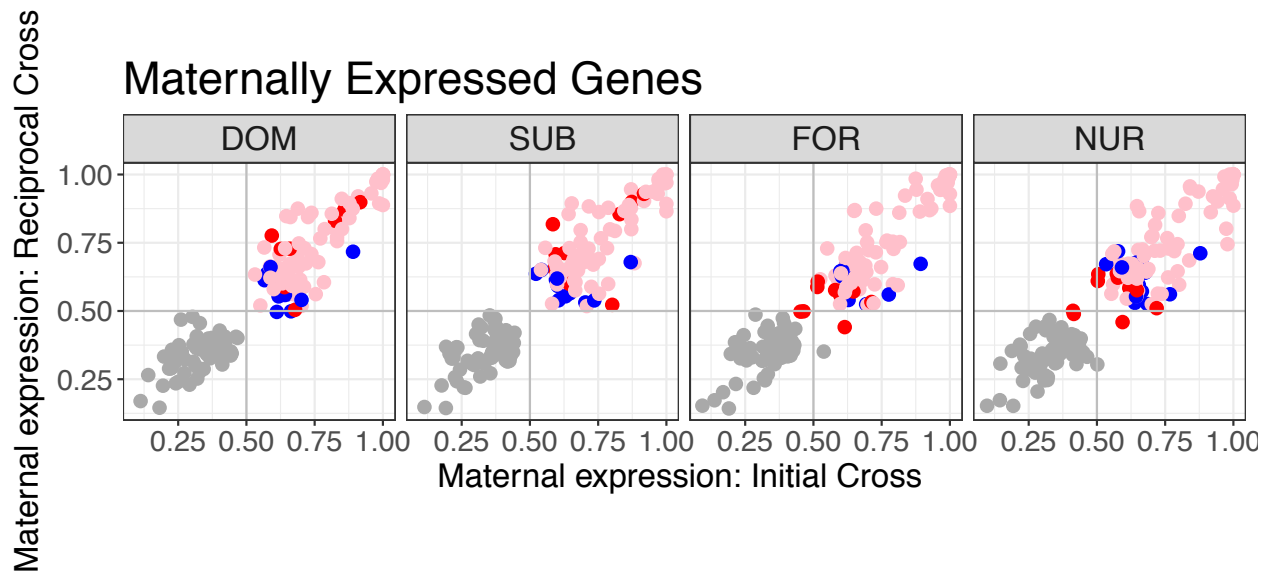
Figure S4: The proportion of maternal expression for each behavioural reproductive type for all genes found to show significant parental expression bias. DOM represents dominant reproductives. SUB represents subordinate reproductives. FOR represents sterile foragers. NUR represents sterile nurses. Each dot represents a gene, the pink dots highlight significantly maternally expressed genes in both sterile and reproductive workers. The red dots are genes showing significant maternal expression bias in reproductive workers only and the blue dots show significant maternal expression bias in sterile workers only.
