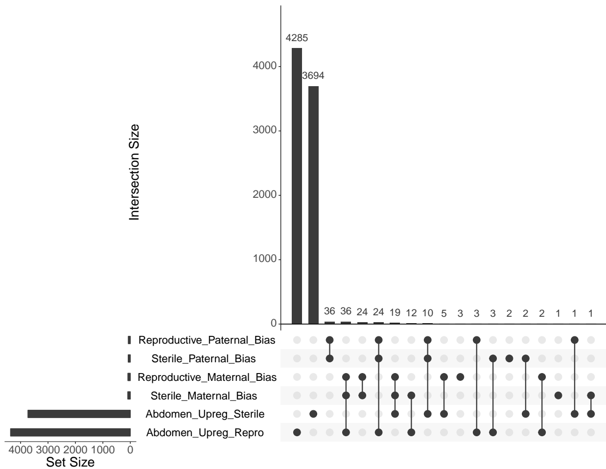
Figure S9: Overlapping genes showing parent-of-origin expression in reproductive (queen-right) and sterile (queen-less) workers with genes showing differential expression in abdomen tissue. The set size indicates the number of genes in each list. The intersection size shows how many genes the corresponding lists have in common. A single dot refers to the number of genes unique to each list.
