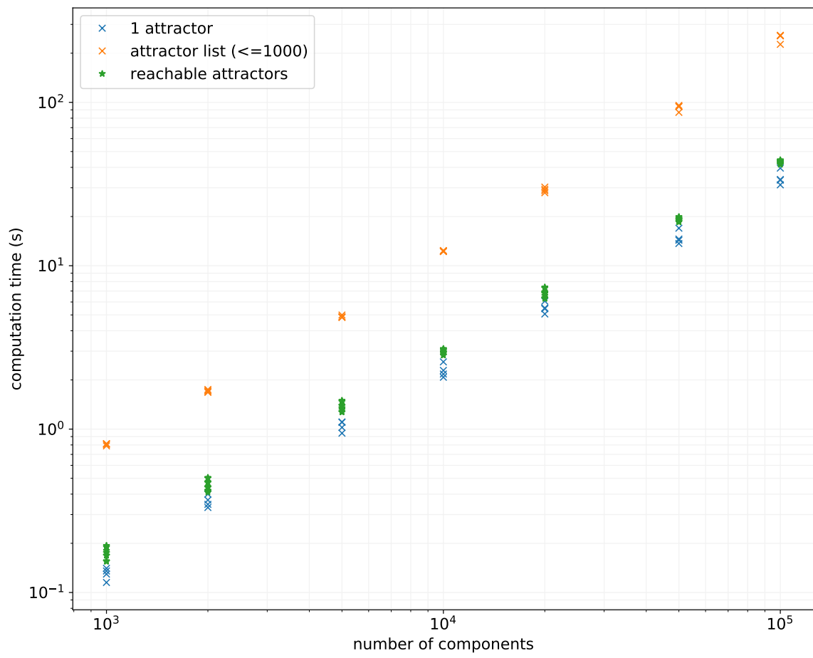
Fig. S4. Computation times on a 3GHz CPU obtained using mpbn software tool on BNs generated with random scale-free influence graph for the computation of a single attractor, the enumeration of 1,000 attractor, and the computation of attractors reachable from random initial conditions. See notebook available at https://nbviewer.jupyter.org/gist/pauleve/b7098fb37cac7e318689e41511d10479 .
