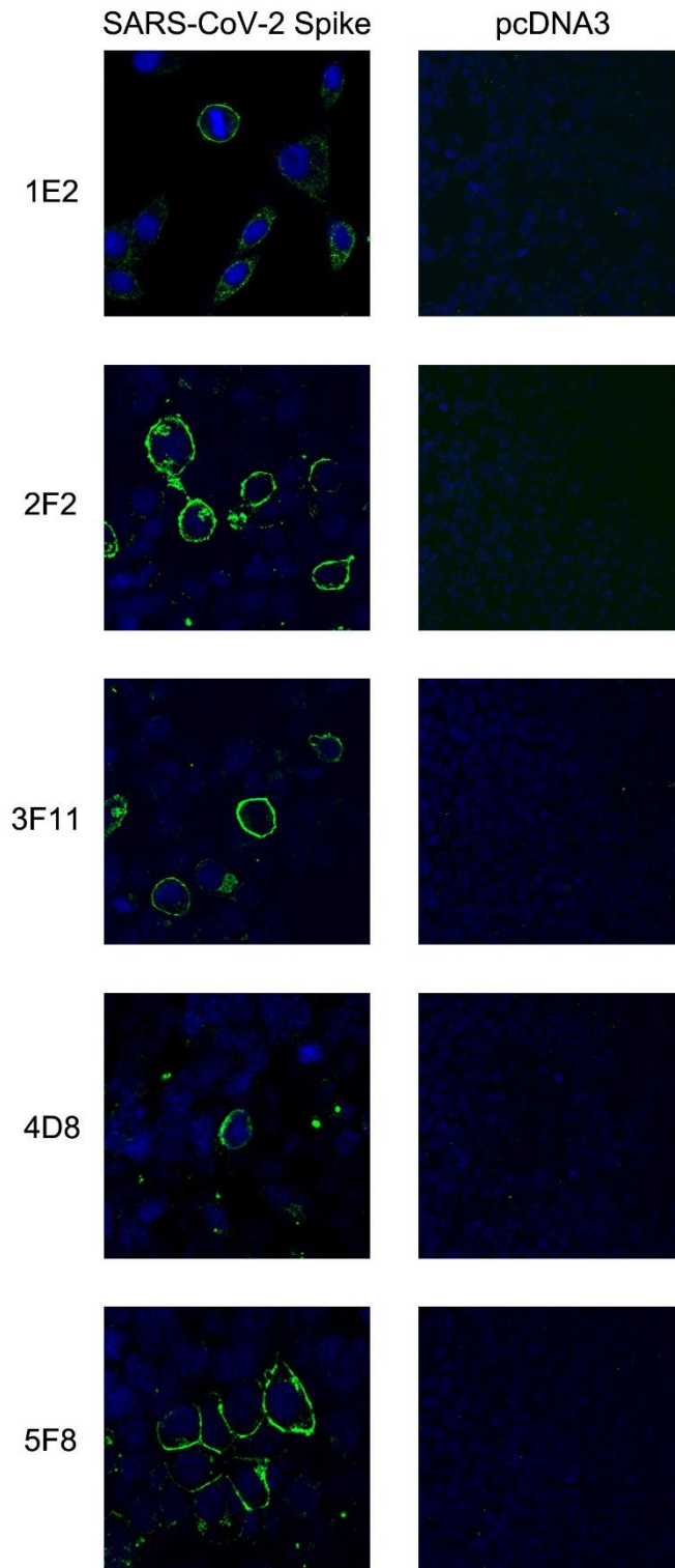
Supplementary Fig. 1. Staining of the transfected SARS-CoV-2 S protein in 293T cells with the sdAbs identified in this study. Overexpressed SARS-CoV-2 S protein was clearly localized on 293T cell plasma membrane.
