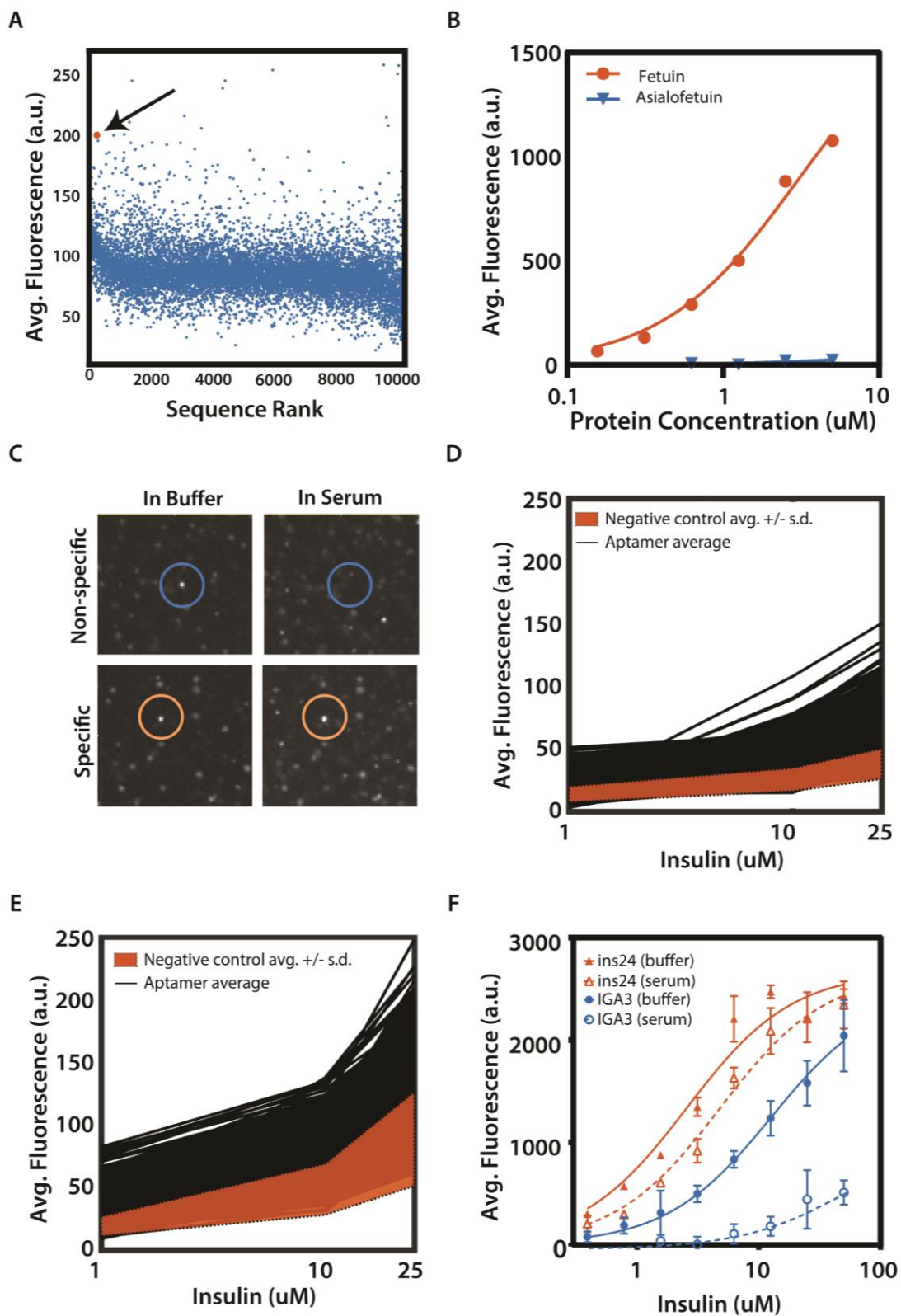
Figure 3 N2A2 can generate base-modified aptamers with excellent specificity. A ) N2A2 measurements of fluorescence intensities of individual aptamer candidates with 1 \mu\text{M} fetuin. Sequences are ranked by
