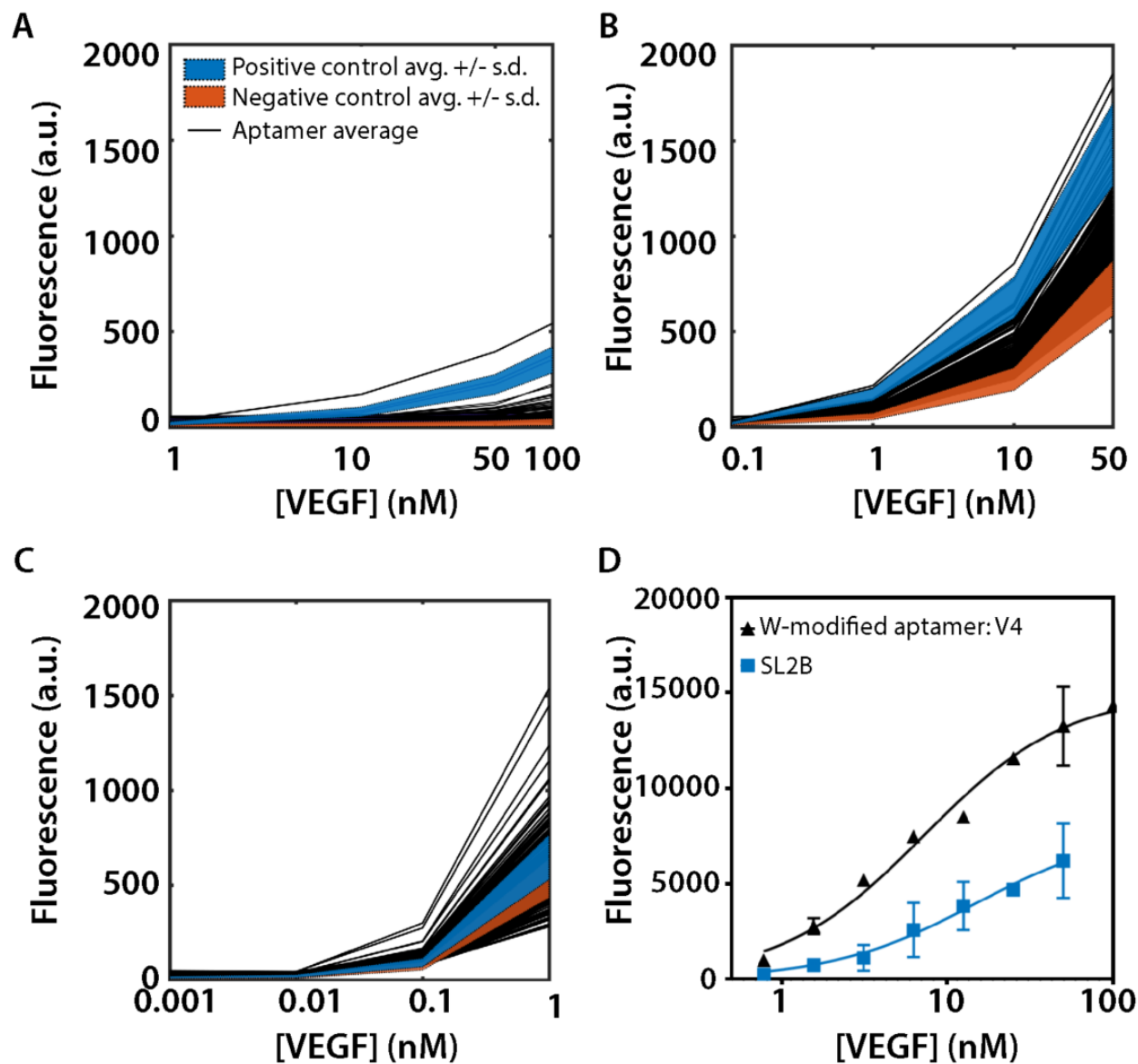
Figure 2. N2A2 screening of aptamer library binding to fluorescently-labeled VEGF. Binding curves are shown for A ) natural DNA, B ) tyrosine (Y)-modified DNA and C ) tryptophan (W)-modified DNA. Black lines show mean binding curves for all unique aptamer candidates. Blue shaded region indicates intensity from the positive control aptamer \pm 1 S.D, and orange shaded region shows background intensity from the negative control sequence \pm 1 S.D. D ) Flow cytometry characterization of a strong VEGF binder identified by N2A2. W-modified aptamer V4 (black) shows greater affinity for VEGF than the positive control aptamer, SL2B (blue).
