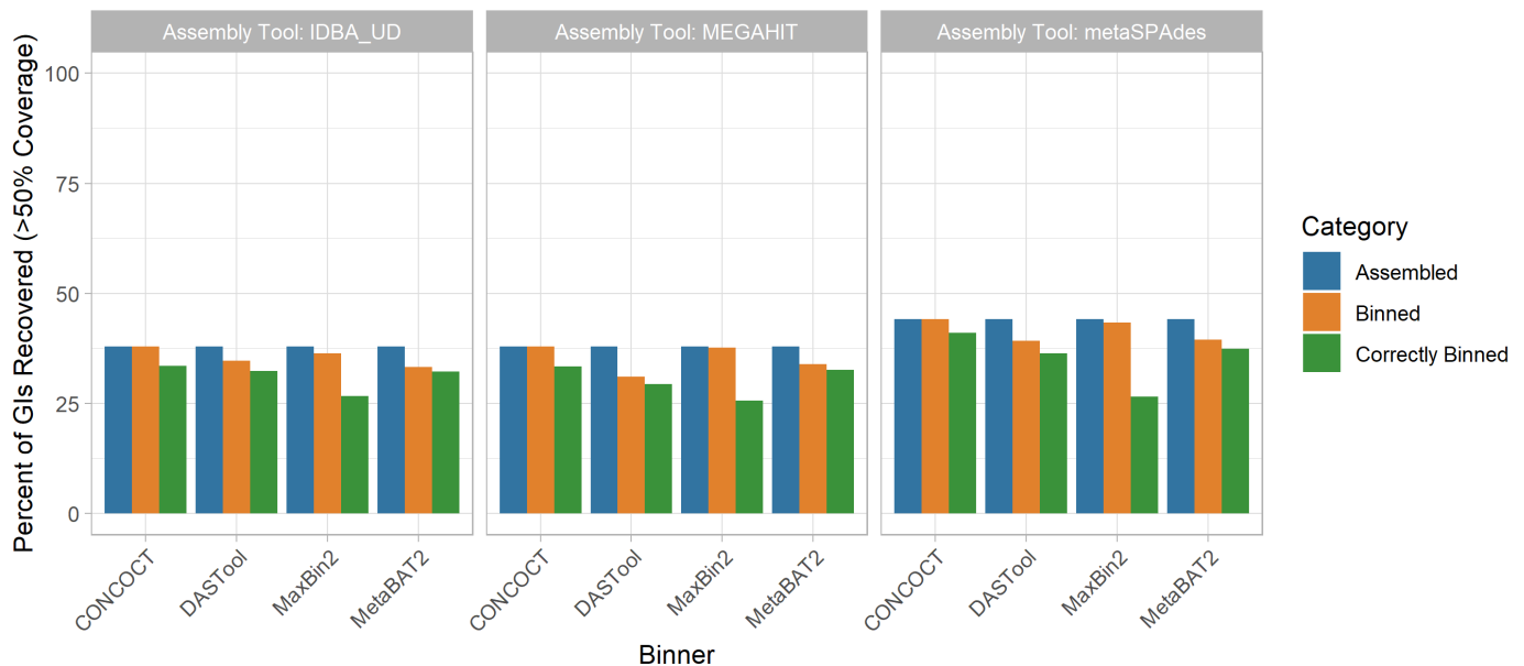
Figure 4: Impact of metagenomic assembly and MAG binning on recovery of GIs. GIs were recovered in a similarly poor fashion to plasmids. Generally, <40% were correctly assigned to the same bin majorly comprised of chromosomal contigs from the same source genome regardless of binning (x-axis) and assembly (panel) methods at >50% coverage. metaSPAdes performed the best at assembling GIs (blue). Maxbin2 and CONCOCT placed GIs in a bin majority of the time (orange) however a very small fraction was correctly binned (green). Generally, GIs were correctly binned better than plasmids with DASTool, MetaBAT2 and CONCOCT.
