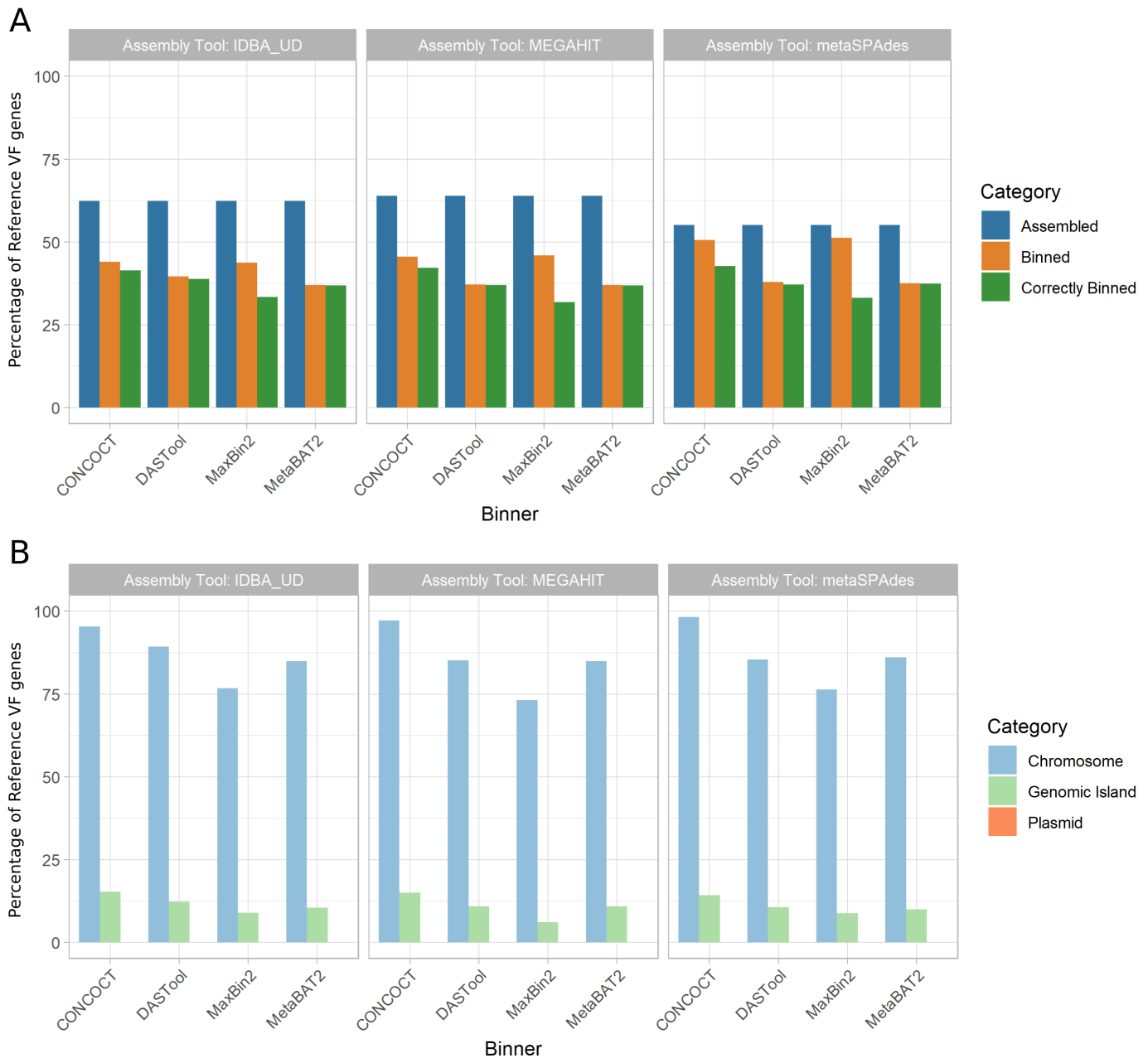
Figure 6: Recovery of VF genes across assemblers, binners, and genomic context. (A) Percent of reference virulence factor (VF) genes recovered across assemblers and binners. The proportion of reference VF genes recovered (y-axis) exhibited a similar trend as AMR genes. Recovery was greatest after the assembling stage (blue), with megahit performing best. Binning tools resulted in a larger reduction in VF genes recovered (orange) compared to AMR genes. However, in the majority of cases, VF genes that are binned are correctly binned (green). metaSPAdes-CONCOCT was again the best performing pair. (B) Percent of correctly binned VF genes recovered in each genomic region. Metagenome assembled genomes (MAGs) were again best at recovering chromosomally located VF genes (light blue), able to correctly bin majority of chromosomally located VFs. GIs recovered again performed very poorly (light green) and again none of the plasmid located AMR genes (orange) was correctly binned.
