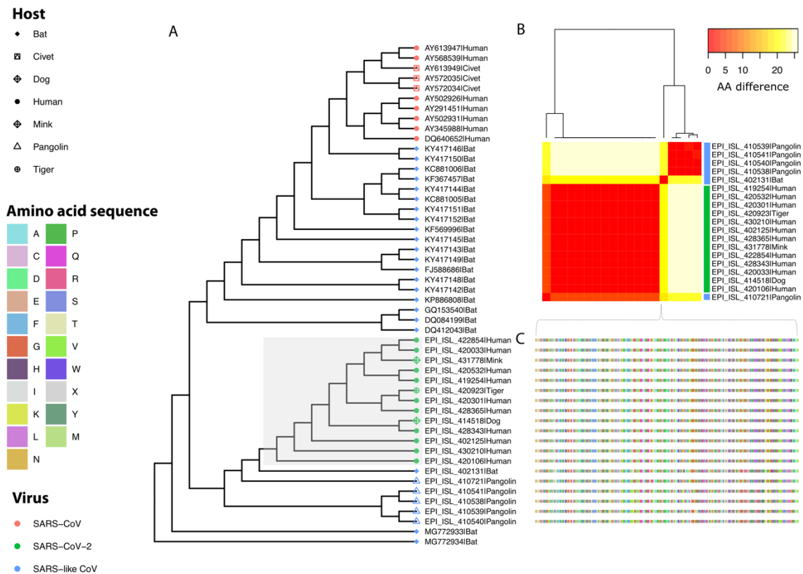
Figure 5: Phylogeny of SARS-like viruses. (a) Genome-wide maximum likelihood phylogenetic tree of SARS-like betacoronavirus strains sampled from diverse hosts (coloured tip symbols; Supplementary Table 3). Genome EPI_ISL_402131 is sample RaTG13 from a horseshoe bat. (b) Pairwise amino acid differences at the S-protein RBD between human and animal strains of SARS-CoV-2, relative to closely related-SARS-like viruses in animal hosts. (c) Sequence alignment for the spike protein receptor binding domain.
