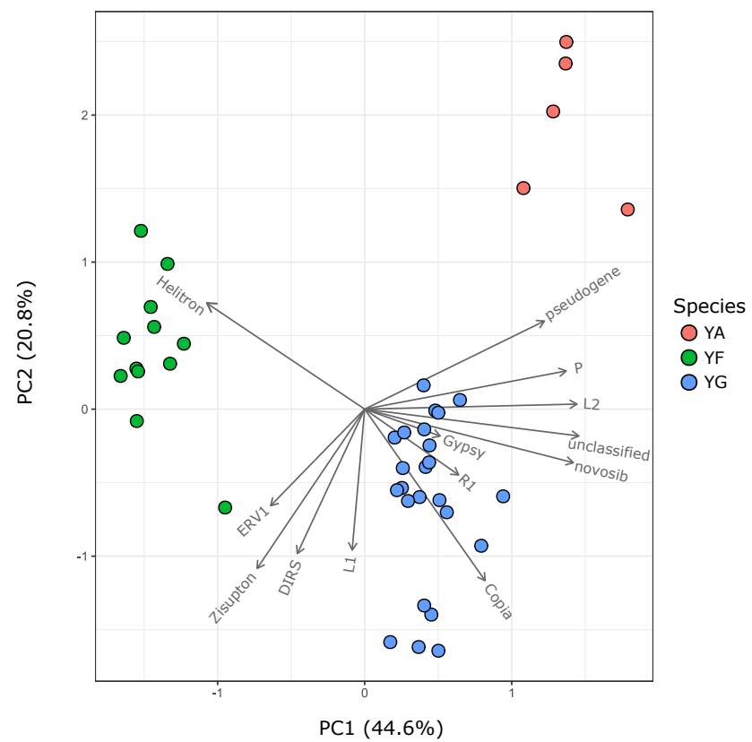
Supplemental Figure 1 - Principal Coordinates Analysis of repeat subfamily abundance in genotypes of three Yucca species.
