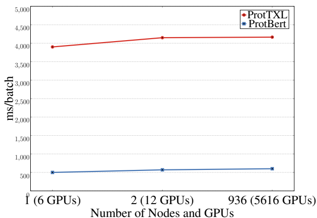
Figure 4: Large Scale Dataset Training: The figure shows the overhead of increasing the number of nodes/gpus for both ProtTXL and ProtBert. The overhead increases slightly from 1 to 2 nodes but remains constant even when scaling up to 936 nodes with a total of 5616 GPUs.
