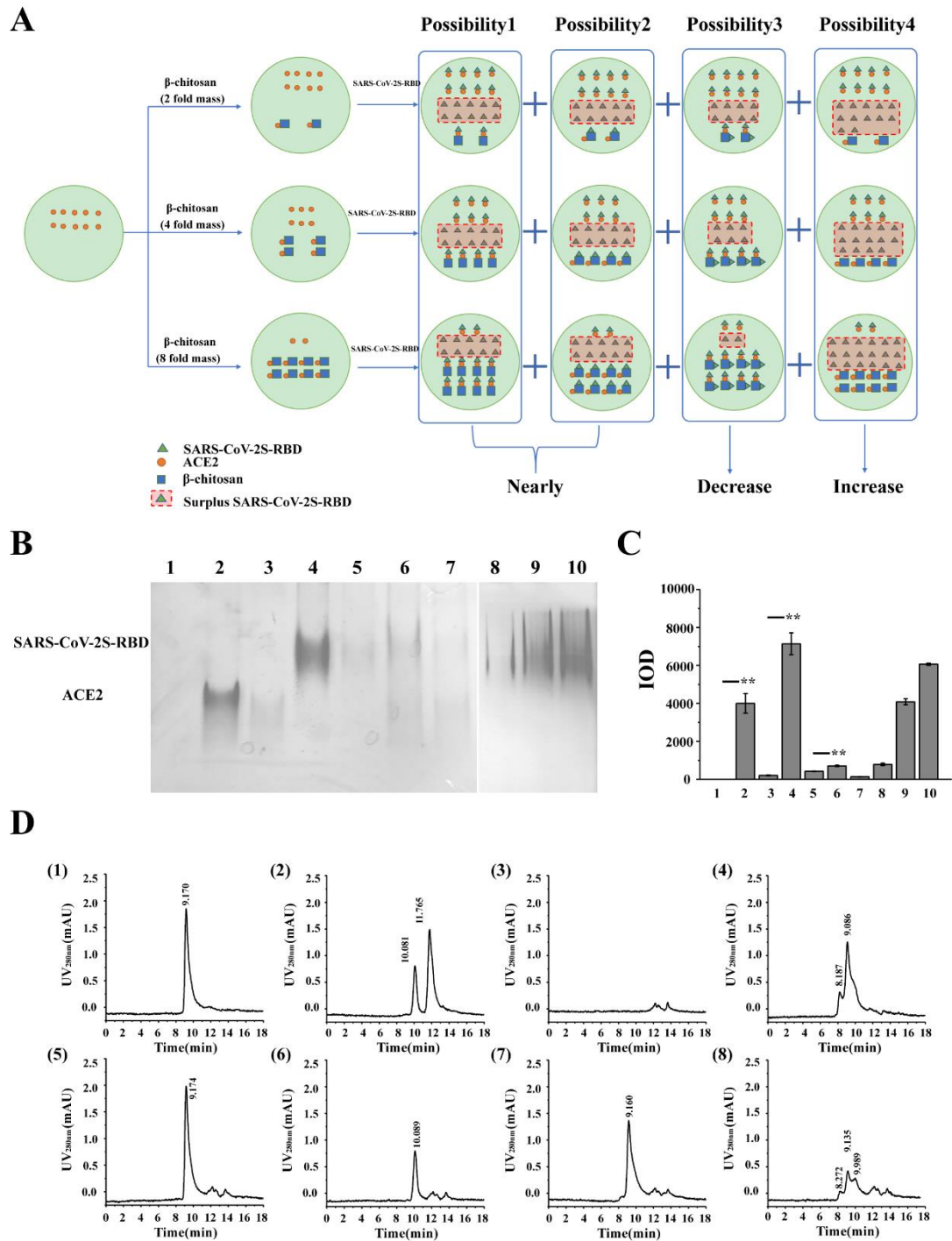
Figure 1. Binding interaction of \beta -chitosan with SARS-CoV-2-S-RBD/ACE2 by Native-PAGE and HPLC analysis.
