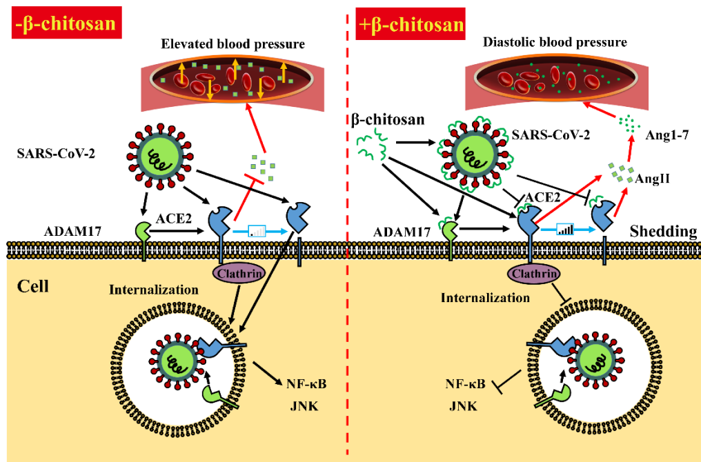
Figure 5 Mechanism of \beta -chitosan against SARS-CoV-2S-RBD/hACE2 binding
