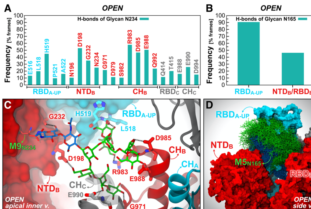
Figure 5. Hydrogen bond interactions of N-glycans at N234 and N165. The main hydrogen bond interactions of N-glycans at N234 ( A ) and N165 ( B ) within the Open system are shown as occupancy across all replicas (% frames). ( C ) A snapshot capturing Man9 glycan at N234 (licorice representation) within NTD-B establishing multiple hydrogen bonds with S protein residues (thicker licorice representation) belonging to RBD-A (cyan surface), NTD-B (red surface), CH-B (red cartoons), and CH-C (gray cartoons). GlcNAc and Man carbons are colored in blue and green, respectively. ( D ) Molecular representation of Man5 glycan at N165 within NTD-B interacting with RBD-A. Multiple (1000) equally interspersed configurations (selected across all replicas) of the glycan at N165 from NTD-B are simultaneously shown. The glycan is represented as colored licorices (GlcNAc in blue, Man in green), whereas RBD-A and NTD-B are represented as cyan and red surfaces, respectively.
