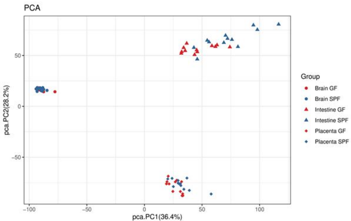
SUPPLEMENTARY Figure 1. Principal component analysis (PCA) of the metabolite profiles of each sample. Component 1 (x axis) explains 36.4% of the variation between the samples and component 2 (y axis) explains 28.2% of the between-samples variation.
