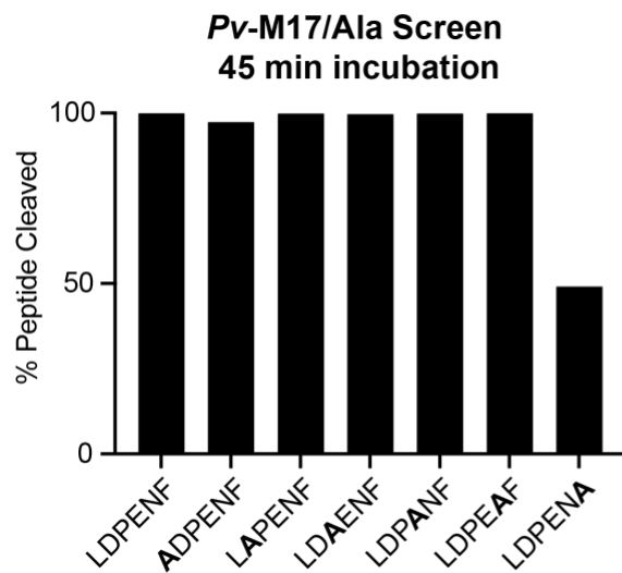
Supplementary Figure S3. Digestion of Ala screen peptides by Pv -M17 and Pb -M17 in 45-min incubation period. Template hexapeptide (LDPENF) and Ala screen peptides were digested to almost 100% in the 45-min incubation period at 37°C. Pv -M17 and Pb -M17 showed decreased activity levels against peptides ADPENF and LDPENA
