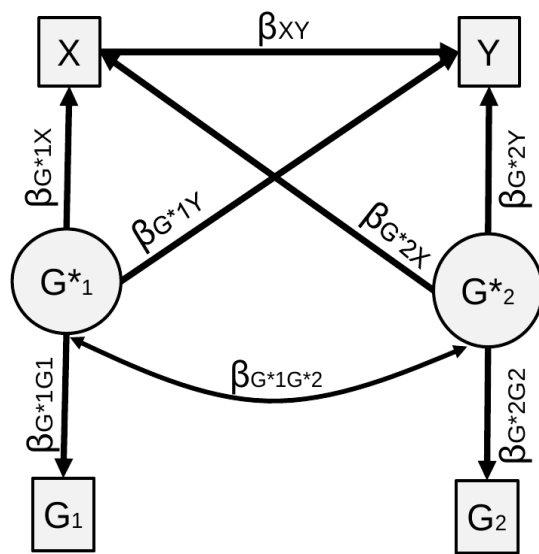
Figure 7: Sensitivity analysis, two polygenic scores.
