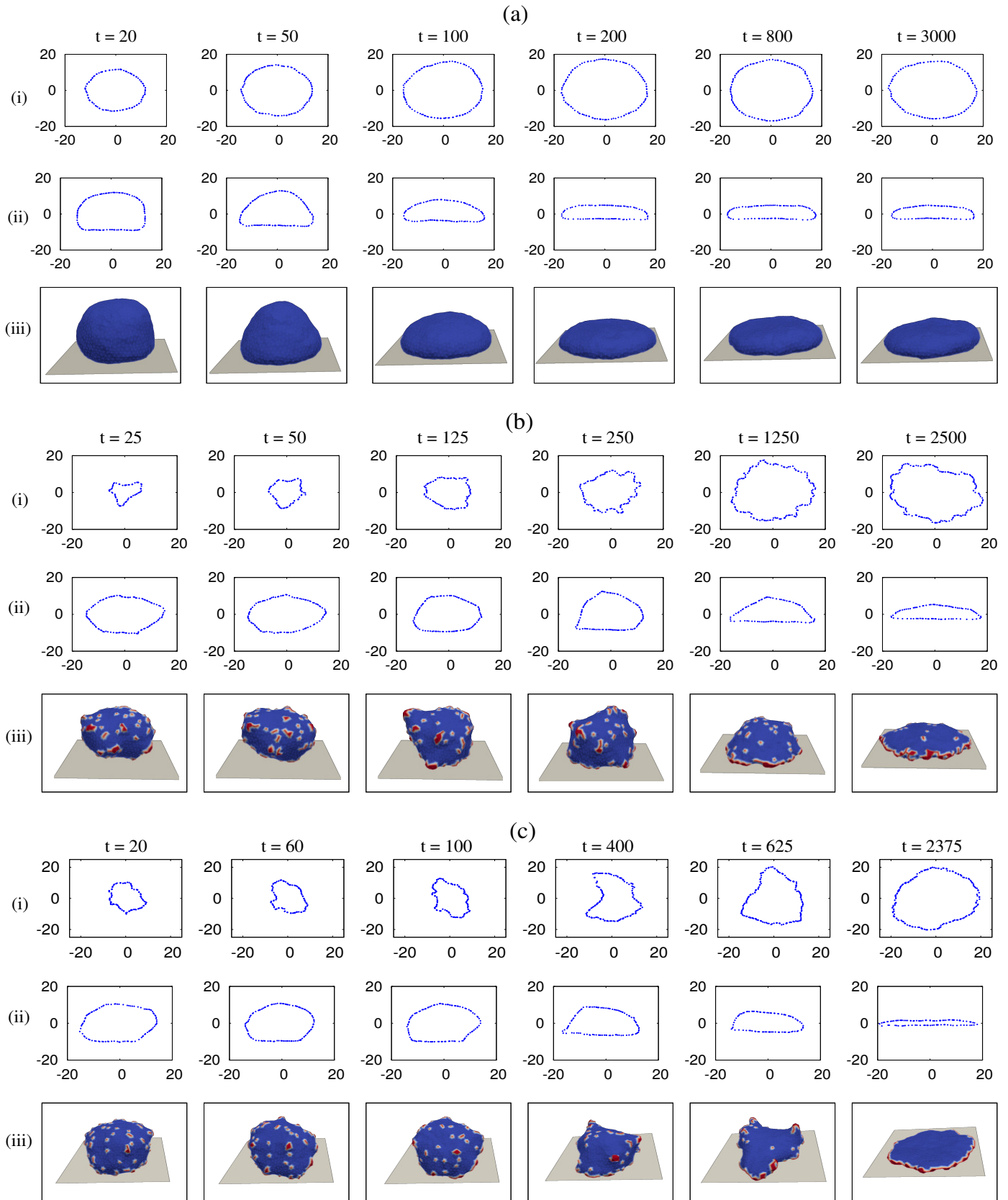
FIG. A-11: Spreading dynamics. (a) Spreading of a protein free vesicle. Here, we choose E_{ad} = 5 k_B T . (i) The bottom view of the adhered area with time, showing that the vesicle adhere quickly. (ii) The side view of the vesicle, showing how the cross-sectional area decreases with the adhesion of vesicles. (iii) Three-dimensional view of the vesicle with time. (b) Spreading of passive vesicle with \rho = 13.82\% and E_{ad} = 0.50 k_B T . Panels (i), (ii) and (iii) are the same as above. The adhered area grows uniformly from the beginning. (c) Spreading of an active vesicle, with \rho = 10.36\% , E_{ad} = 0.50 k_B T and F = 4 k_B T / l_{min} . In the beginning, the growth of adhered area is slow, then accelerates and finally the vesicle takes the shape of a pancake. The unit of time (t) is taken as 2 \times 10^3 MC steps.
