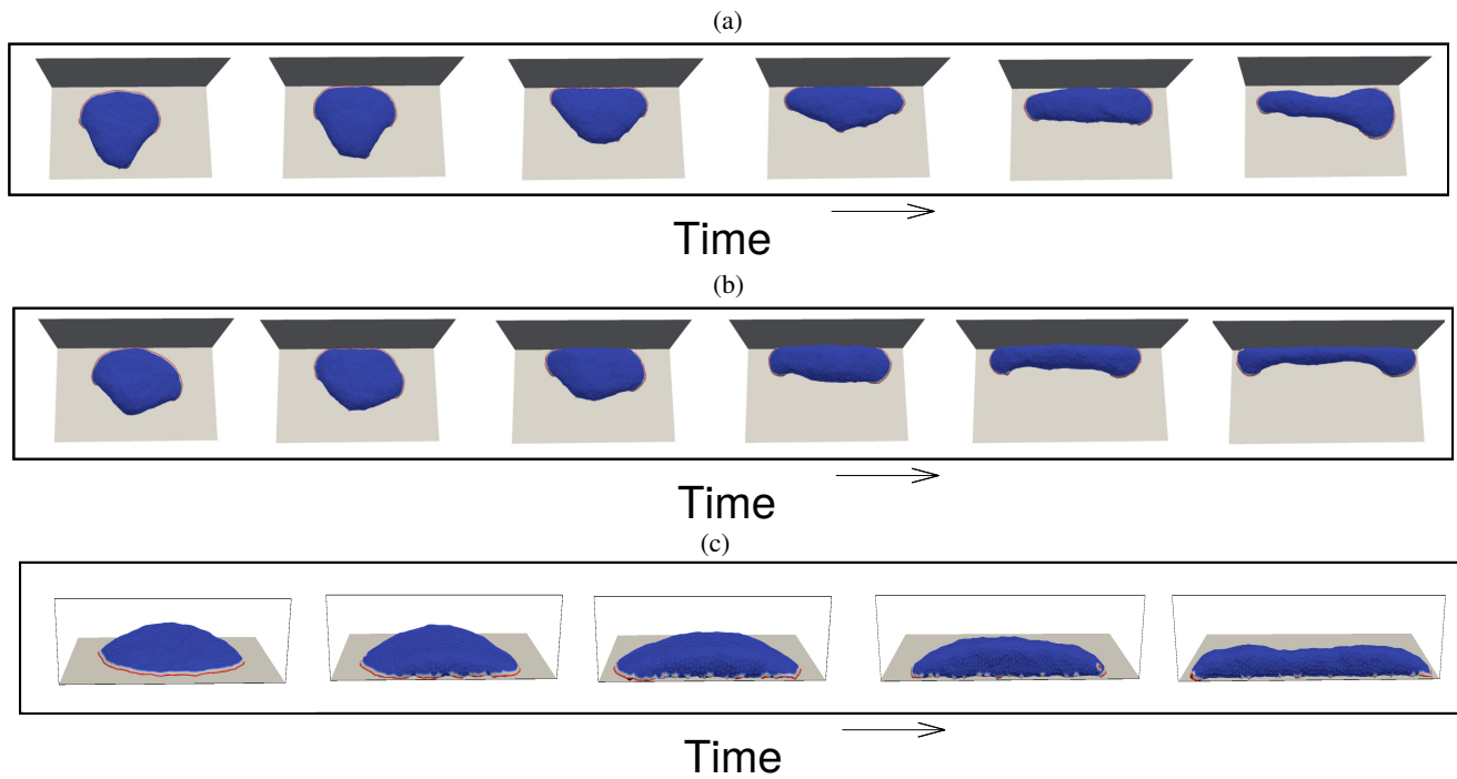
FIG. A-18: Motile vesicle growing against an immobile barrier. (a) We plot the snapshots of vesicle with time for a non-adhesive barrier. (b) The snapshots of the vesicle with time for an adhesive barrier. (c) The side view of the vesicle for the adhesive case. We note that in both the adhesive and non-adhesive cases, the crescent-shaped vesicle breaks into two-arc shape. Here, we use \rho = 3.45\% , F = 4 k_B T / l_{min} and E_{ad} = 3.0 k_B T . For the adhesive barrier also, we use E_{ad} = 3.0 k_B T .
