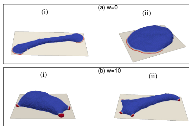
FIG. A-16: Snapshots of vesicle with various values of protein-protein interaction strength w . (a) For w = 0 k_B T , we obtain the two-arc and crescent-like shapes as found for the case of w = 1 k_B T (Fig.9). For (i), we use E_{ad} = 2.0 k_B T , F = 4.0 k_B T/l_{min} and \rho = 3.45 \% , and for (ii), we use E_{ad} = 3.0 k_B T , F = 2.0 k_B T/l_{min} and \rho = 3.45 \% . (b) For very large w = 10 k_B T , the vesicle forms small isolated clusters, that do not break-up or merge after long time. Here, for (i), we use E_{ad} = 2.0 k_B T , F = 3.0 k_B T/l_{min} and \rho = 3.45 \% , and for (ii), we use E_{ad} = 2.0 k_B T , F = 4.0 k_B T/l_{min} and \rho = 3.45 \% .
