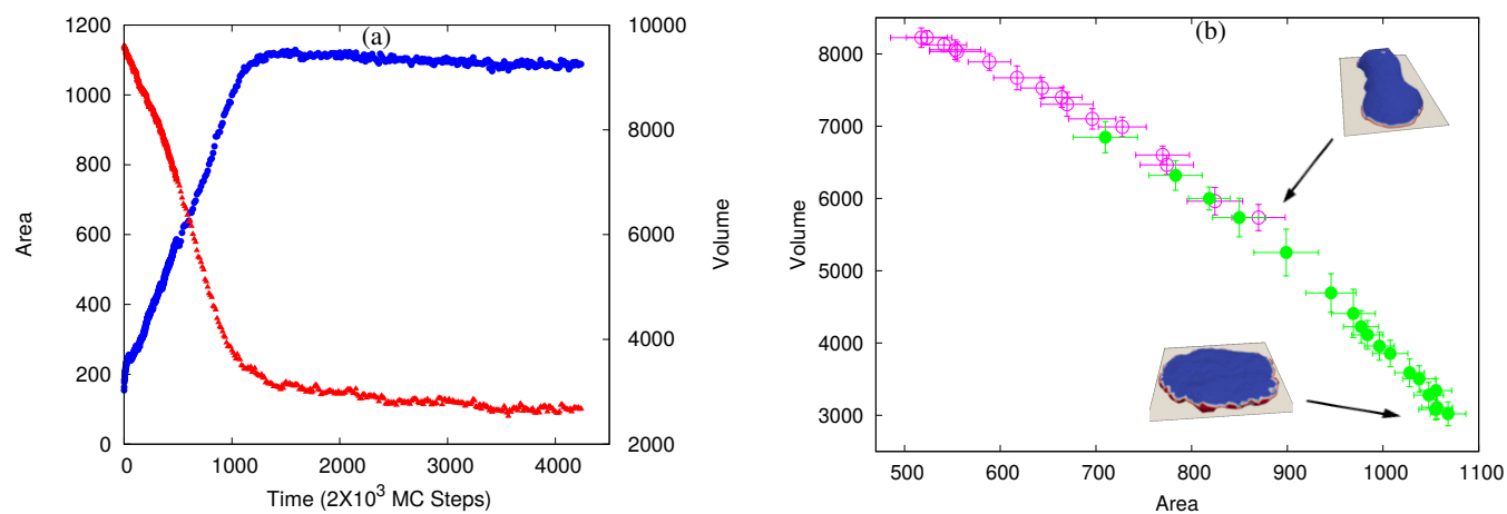
FIG. A-13: Area-Volume relation. (a) The variation of area and volume with time for an active vesicle. The red triangles are for the volume and the blue circles are for the area. We use here, \rho = 10.36 \% , E_{ad} = 0.50 k_B T and F = 4 k_B T / l_{min} . (b) The area-volume relation in the steady state for active case with E_{ad} = 0.50 k_B T and two different values of \rho . The hollow magenta circles are for \rho = 4.84 \% and the green solid circles are for \rho = 10.36 \% . We also show the snapshot of vesicles for both the \rho , for their highest area. Here, we vary F in order to access different area and volume in the steady state. We note that for larger \rho (which corresponds to the pancake shape), the system can access larger area and smaller volume in comparison to lower \rho (which corresponds to the two-arc elongated shapes).
