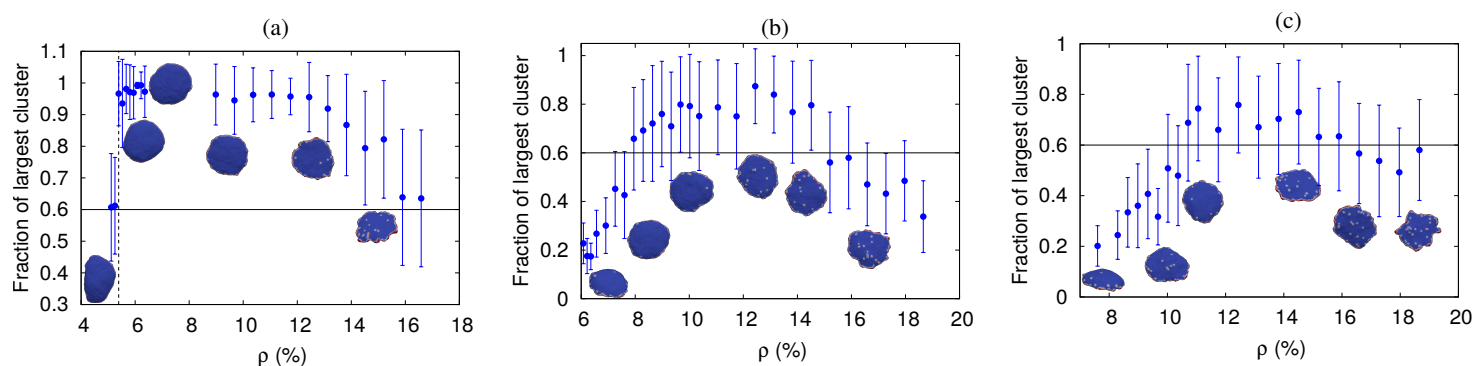
FIG. A-12: Fraction of largest cluster with \rho for various values of F and E_{ad} = 0.50 k_B T . (a) F = 2.0 k_B T / l_{min} , (b) F = 1.0 k_B T / l_{min} , and (c) F = 0.50 k_B T / l_{min} . The vertical dashed line of (a) is showing the pancake transition, which is a sharp transition. For (b) or (c), the pancake transition is not very sharp, and the shape is assumed to be a pancake when the size of largest cluster is at least 60 % of the total number of proteins.
