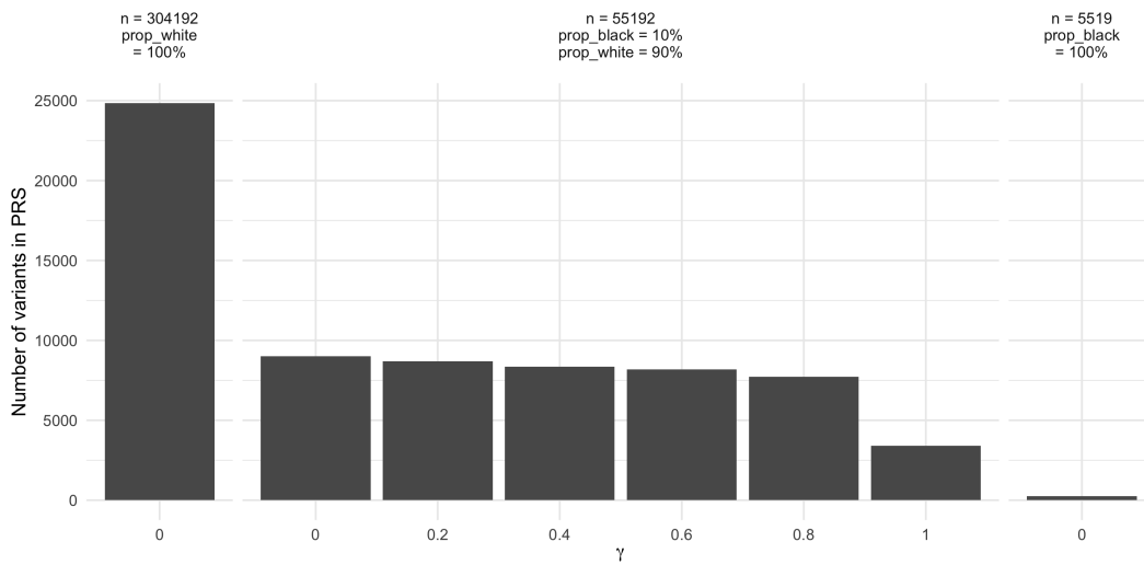
Figure 2: Number of variants with non-zero effect estimates in the polygenic risk scores for height.
