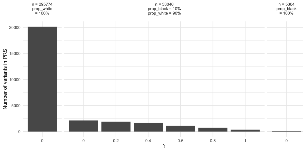
Figure 1: Number of variants with non-zero effect estimates in the polygenic risk scores for mean corpuscular volume.
