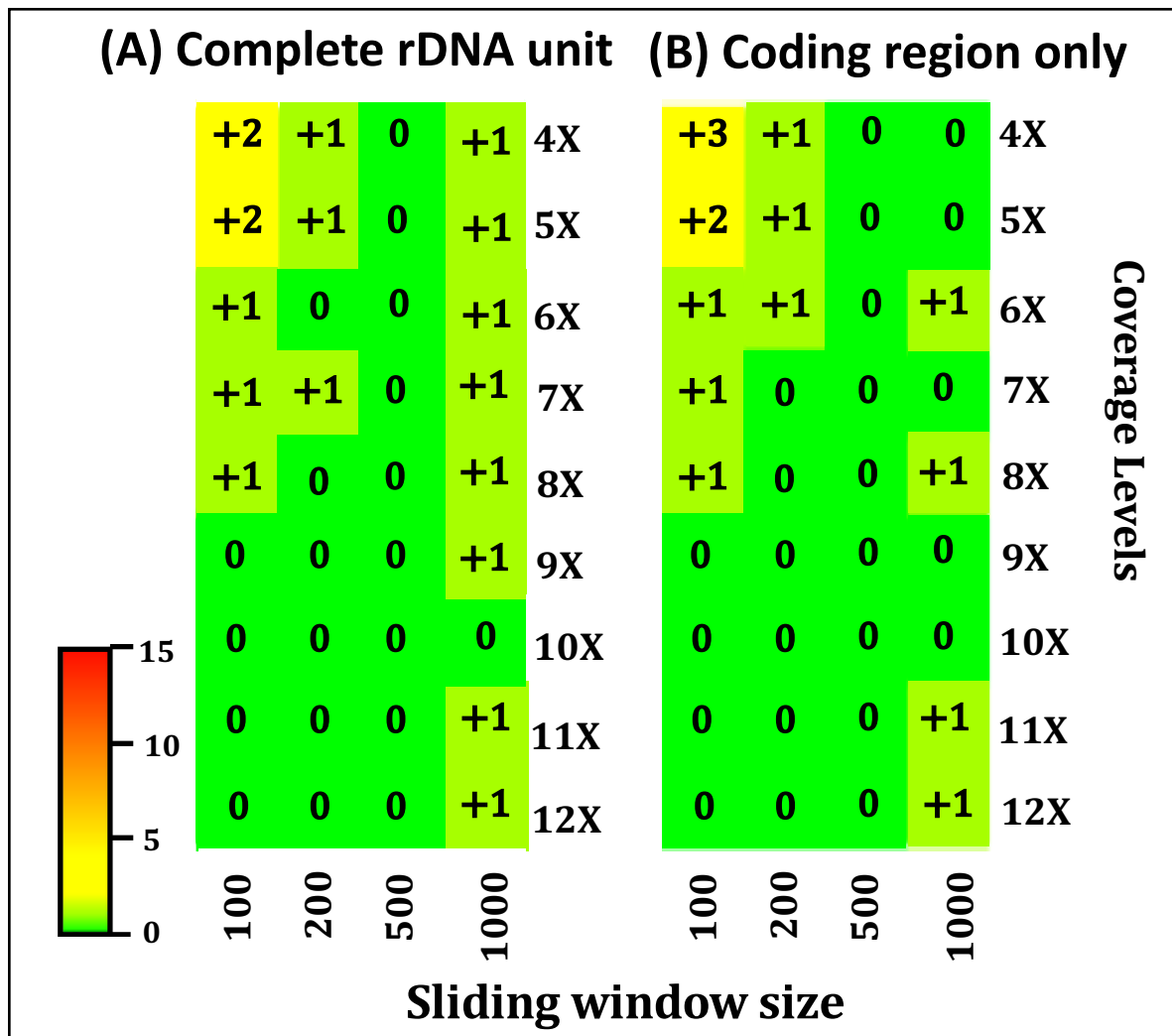
Supplementary Figure 3. Copy number estimates are similar when only using the rRNA coding region. Each cell represents the deviation of the calculated modal rDNA copy number from 20 for each coverage level and sliding window size combination. (A) uses coverage information from the whole rDNA repeat, while (B) only uses the information from the rRNA coding region. The heatmap scale used is indicated and deviations are rounded to the nearest integer.
