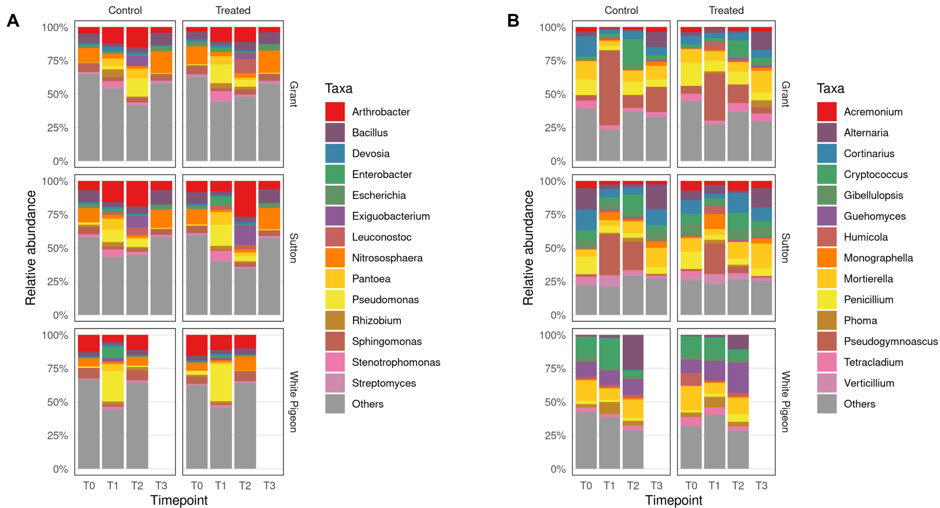
Figure S1. Taxonomic composition of soil samples across locations and sampling times. (A) Most abundant bacterial genera identified. (B) Most abundant fungal genera identified. T0 - before planting; T1 - one month after planting; T2 - two months after planting; T3 – after harvest.
