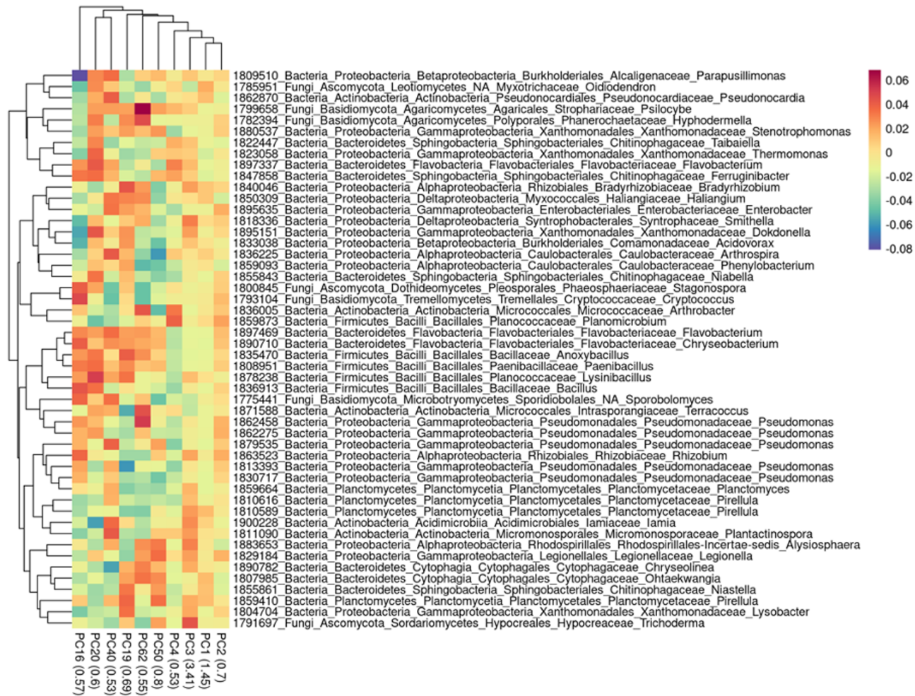
Figure S2. Taxonomic assignment and their relationship with yield (fold change values) of the OTUs contributing to the ten most important principal components of the beta-diversity ordination generated for the yield predictive model.
