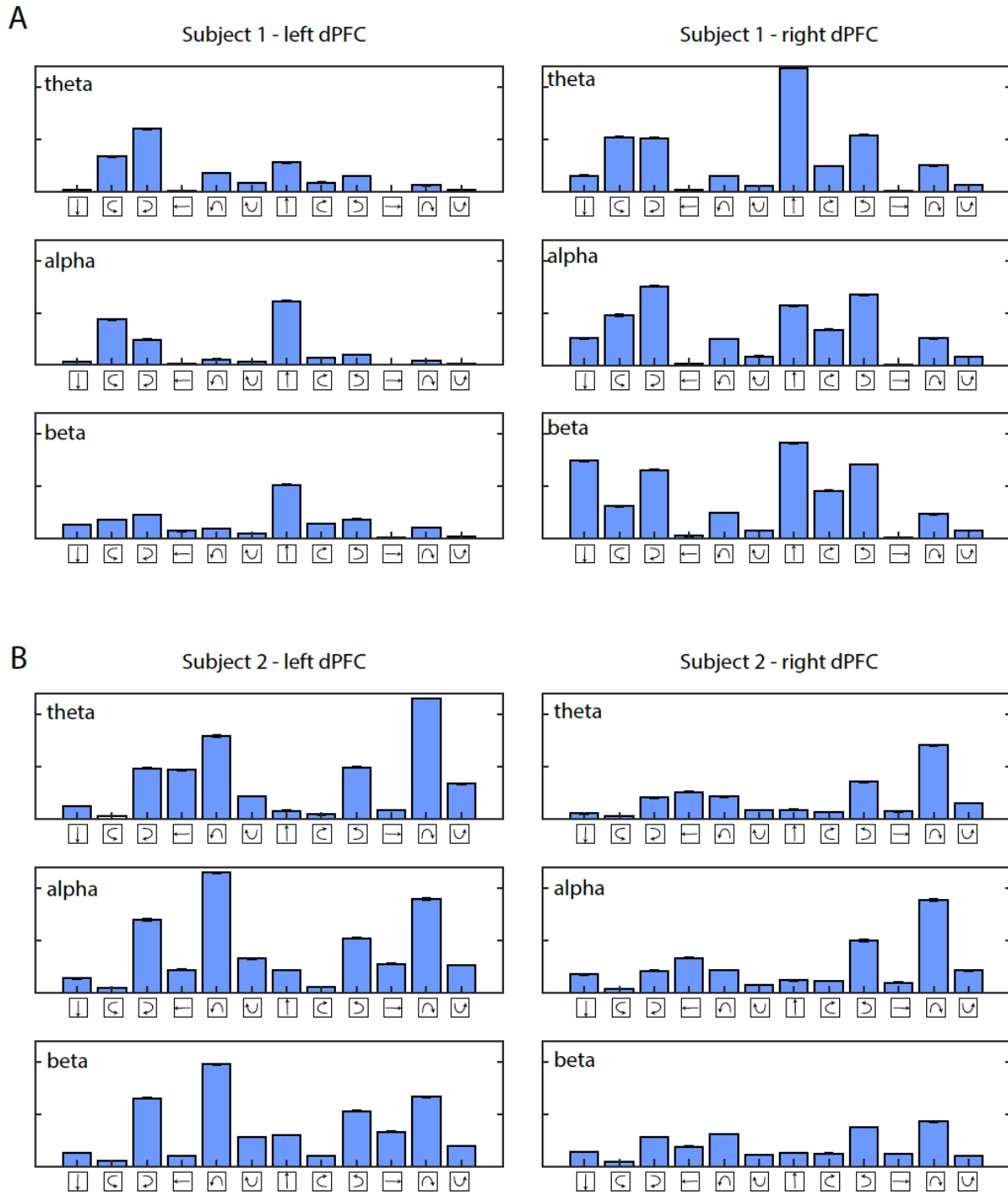
Supplemental Fig. 2: (A, B) Number of wave instants observed for different wave types across frequencies and arrays.
