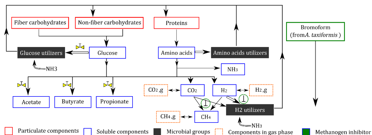
Figure 1. Representation of the rumen fermentation model (adapted from (Muñoz-Tamayo et al. , 2016)). Hydrolysis of carbohydrates (fiber and non-fiber) and proteins releases respectively sugars and amino acids soluble monomers which are further utilized by the microbiota. The utilization of substrate is directed to product formation (single arrows) and microbial growth (double arrows). Each substrate is utilized by a single microbial functional group. The bromoform contained in A. taxiformis produces a direct inhibition of the growth rate of methanogens that results in a reduction of methane production and in an accumulation of hydrogen. The symbol ⊥ indicates the direct effect of the bromoform on the methanogenesis. Hydrogen exerts control on sugars utilization and on the flux allocation towards volatile fatty acids production. The symbol ⊣ indicates the hydrogen control effect on the rumen fermentation.
