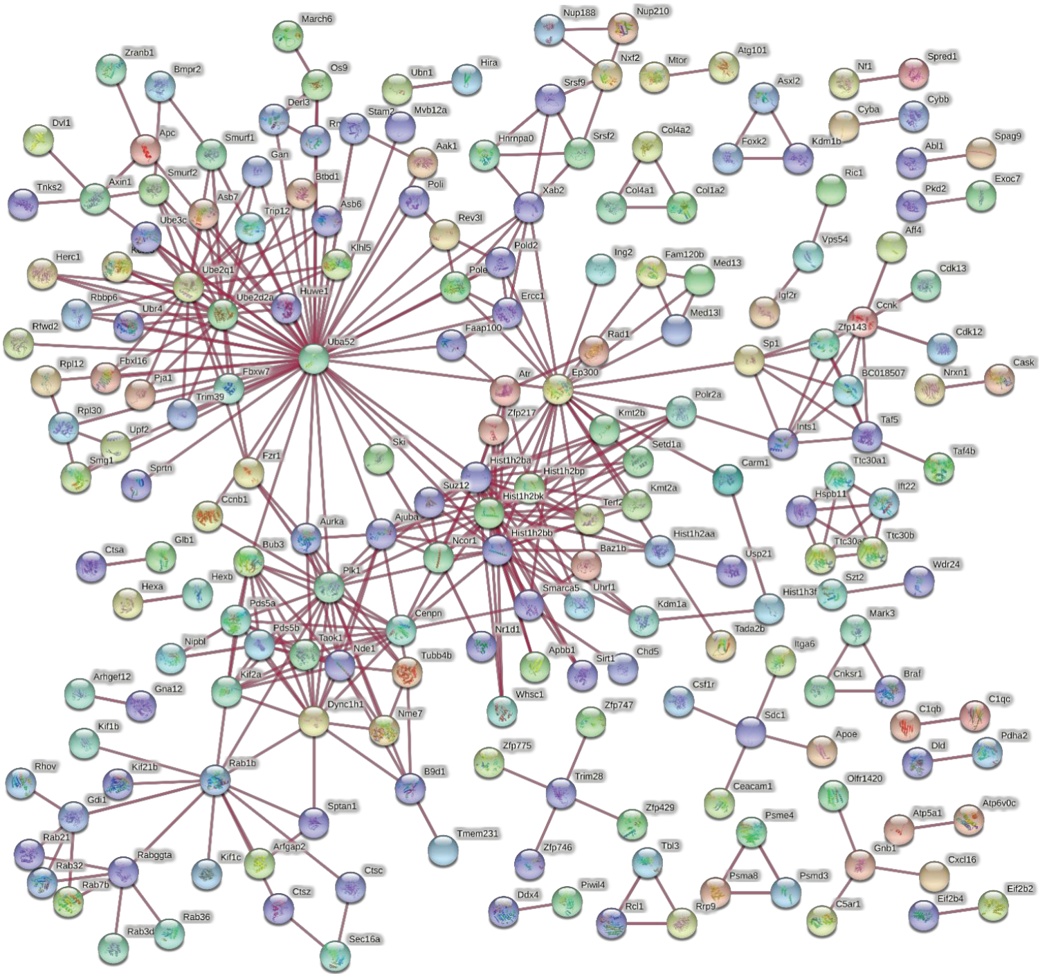
Figure S3. Protein-protein interactions (PPIs) of E16.5 DEGs. Plot generated by STRING of DEGs from E16.5 RNA-seq that had at least one PPI (physical network, highest confidence) (Szklarczyk et al. 2019). There was a significant enrichment of PPIs ( p < 0.01 ).
