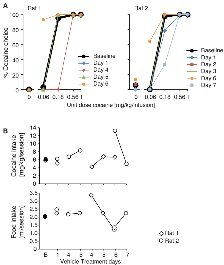
(A) Percent cocaine choice allocation in two rats that received repeated vehicle injections, all days tested; rat 1 started on a Friday, rat 2, on a Wednesday. (B) Session-wide cocaine and food intakes in each rat as a function of successive days (baseline levels shown as filled symbols, treatment days as open symbols; baseline level symbols overlap).
