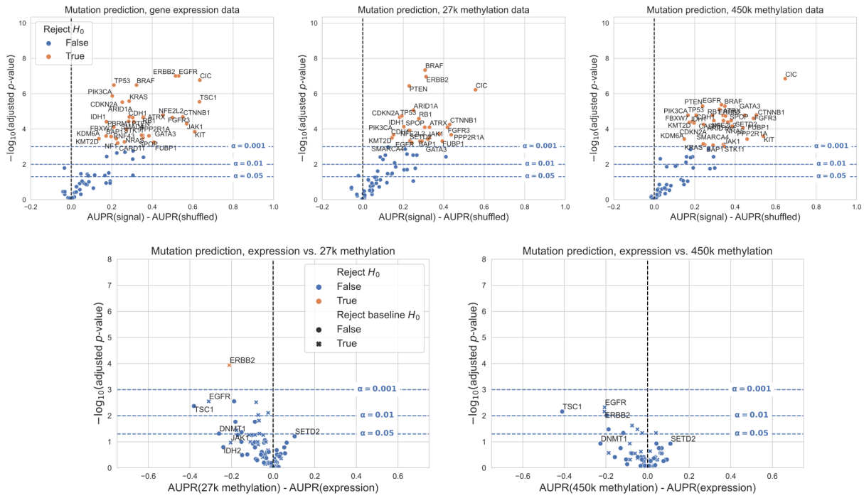
Figure 10: Volcano-like plots showing predictive performance for each gene in the Vogelstein et al. gene set for expression and DNA methylation, on the sample set used for the “all data types” experiments. The first row shows performance relative to the permuted baseline, and the second row shows direct comparisons between data types. The x-axis shows the difference in mean AUPR compared with a baseline model trained on permuted labels, and the y-axis shows p -values for a paired t -test comparing cross-validated AUPR values within folds.
