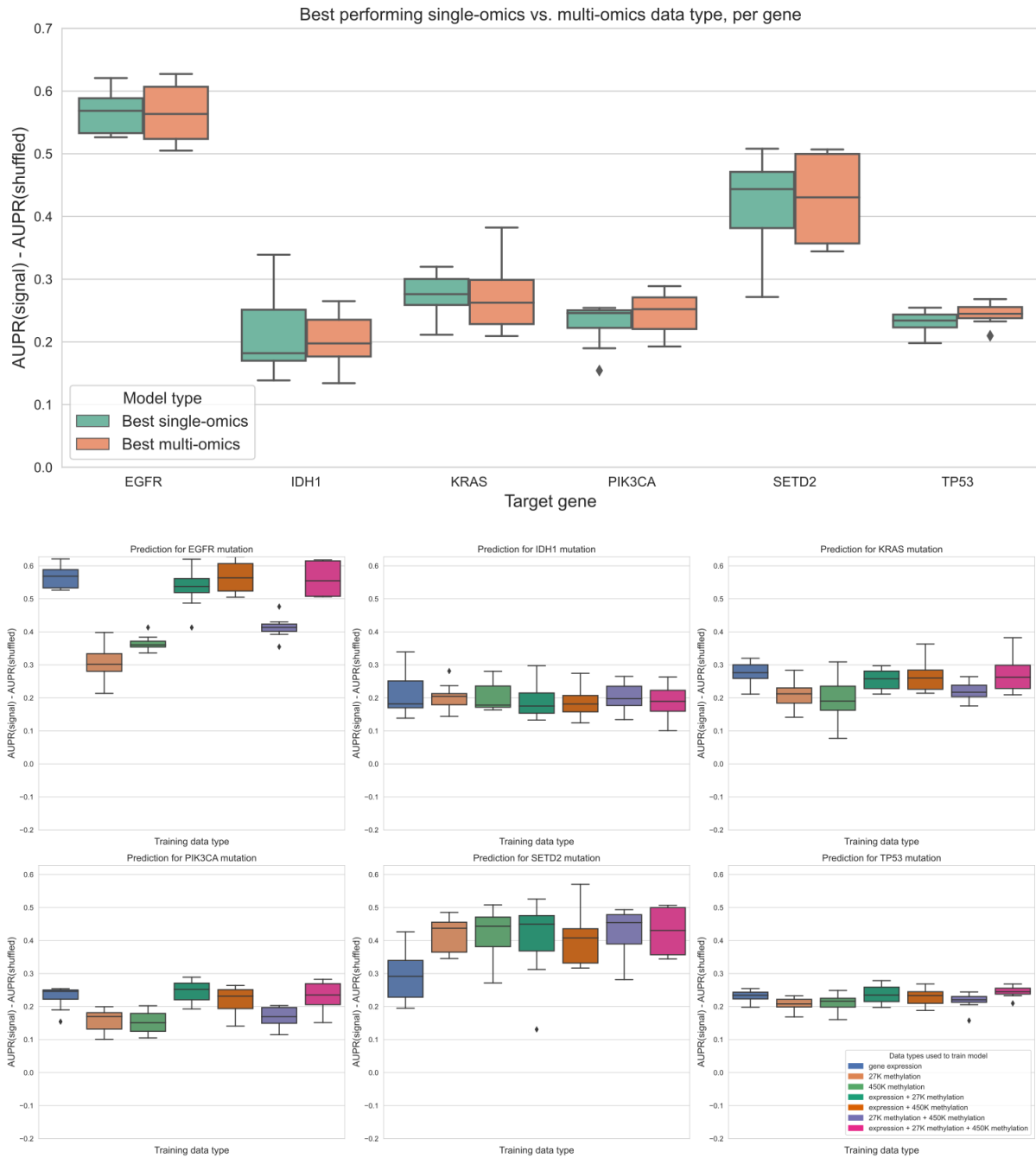
Figure 13: Top plot: comparing the best-performing model (i.e. highest mean AUPR relative to permuted baseline) trained on a single data type against the best “multi-omics” model for each target gene, using raw (not PCA compressed) features. For feature parity between data types, the top 20,000 features by mean absolute deviation were used for each data type. The difference between single-omics and multi-omics performance for TP53 was statistically significant ( p=0.0078 ), but other differences between single-omics and multi-omics models were not statistically significant using paired-sample Wilcoxon tests across cross-validation folds, for a threshold of 0.05. Bottom plots: classifier performance, relative to baseline with permuted labels, for individual genes. Each panel shows performance for one of the six target genes; box plots show performance distribution over 8 evaluation sets (4 cross-validation folds x 2 replicates).
