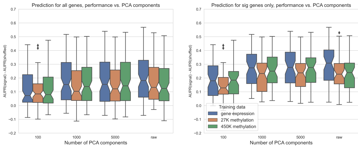
Figure 11: Predictive performance for genes in the Vogelstein et al. gene set, using each of the three data types as predictors. The x-axis shows the number of PCA components used as features, “raw” = no PCA compression.
