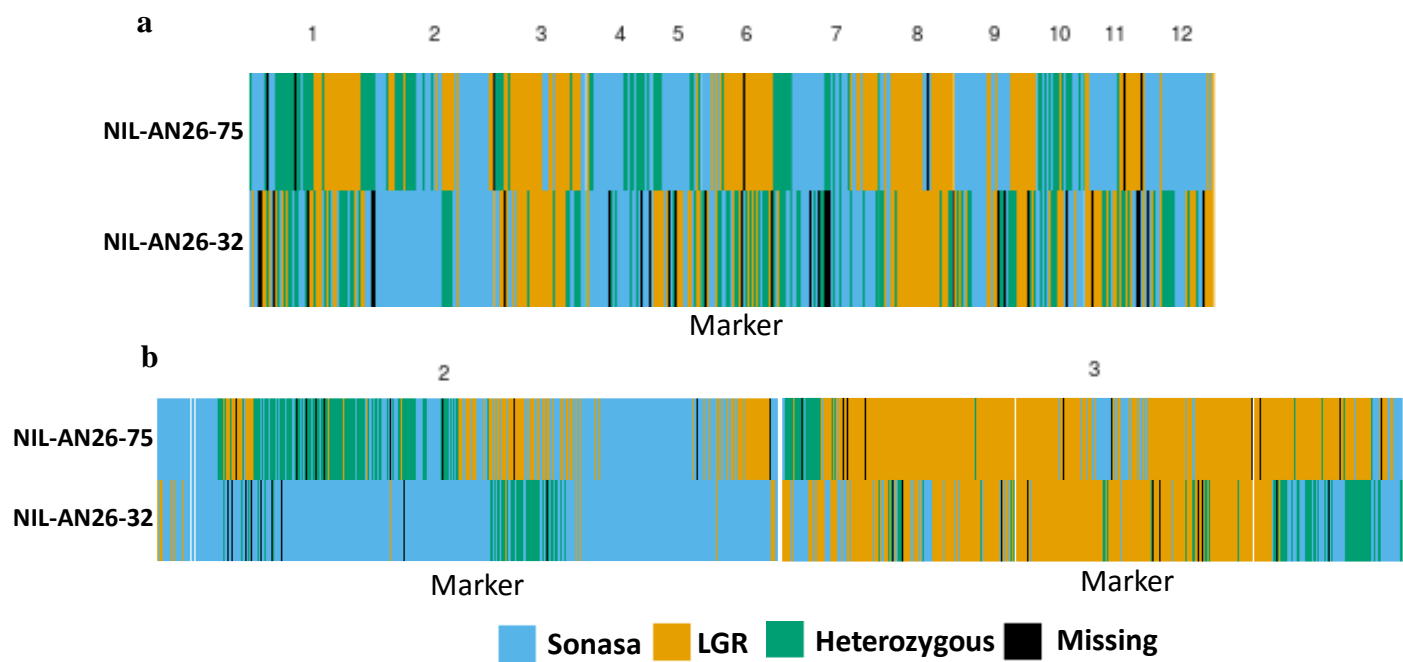
Supplementary Figure 11. Background analysis of two Sonasal \times LGR BC 4 F 1 lines. a) Graphical of Genotype of all 12 rice chromosome, and b) Graphical of Genotype of chromosome 2 and chromosome 3.
