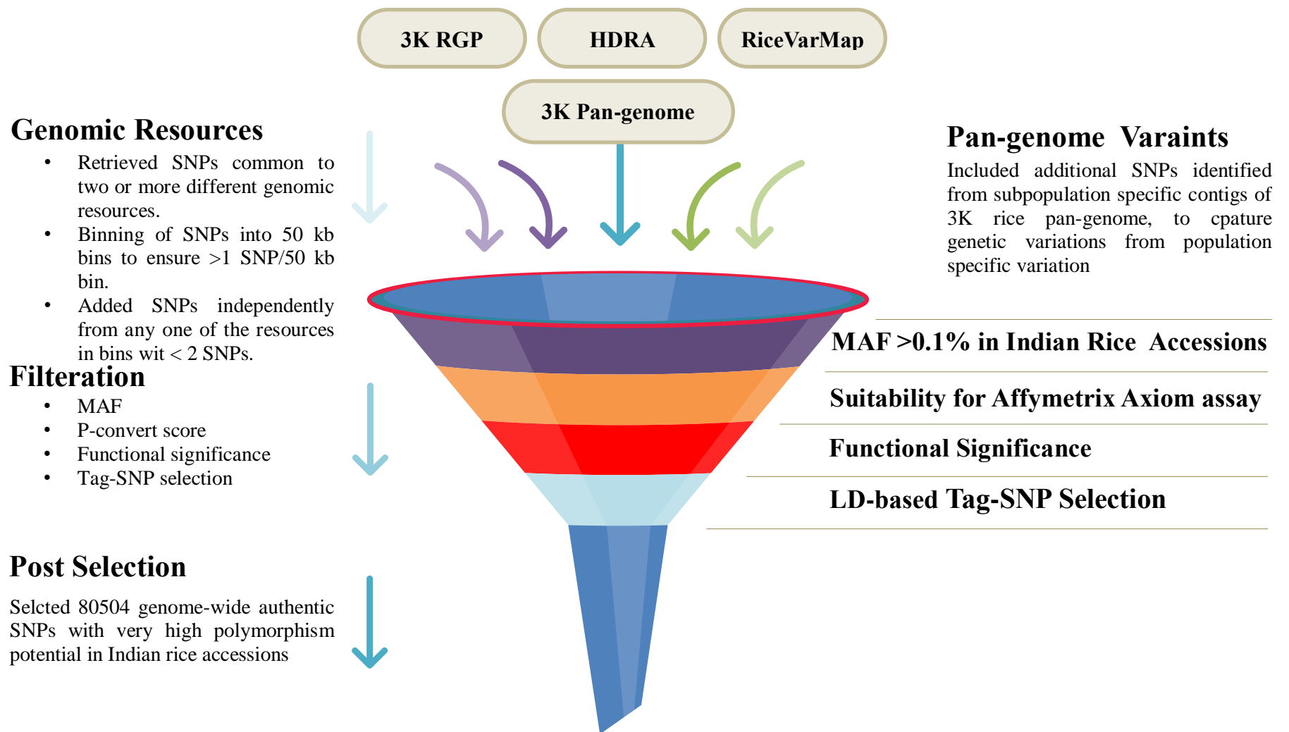
Supplementary Figure 13. Workflow describing steps involved in designing of Rice Pan-genome Genome Genotyping Array (RPGA). 3K RGP: 3K Rice Genomes Project, HDRA: High-Density Rice Array, MAF: Minor Allele Frequency
