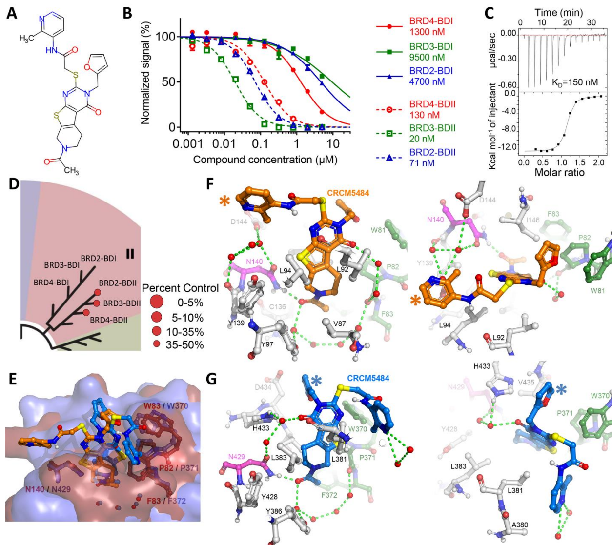
3 4 Figure 3. Characterization of CRCM5484. (A) Chemical structure. (B) HTRF selectivity assay on the BDI (solid lines) and BDII 5 (dashed lines) of BRD2 (blue), BRD3 (green) and BRD4 (red). (C) Representative Isothermal Titration Calorimetry (ITC) 6 experiment with CRCM5484 in the cell and BRD3-BDII in the syringe at 15°C. (D) BROMOscan data (DiscoverX) on the 8 BET 7 bromodomains families. (E) Superposition of the co-crystal structures of CRCM5484 (orange)/BRD4-BDI (red) (PDB: 7Q3F) and 8 CRM5484 (cyan) / BRD2-BDII (blue) (PDB: 7Q50). Water molecules are shown as red and blue spheres for the BRD4-BDI and 9 BRD2-BDII complexes, respectively. F and G) Co-Crystal structures of CRCM5484 with BRD4-BDI (Orange) and BRD2-BDII (Blue) 10 showing the hydrogen bond interactions as green dotted lines, the canonical asparagine binding residue as magenta, the WPF 11 shelf as green and the rest of the domain as white balls and sticks. The picoline (orange *) and furan moiety (blue *) showed 12 poor electronic density and their positioning were driven by geometry and residual electron density during refinement.
