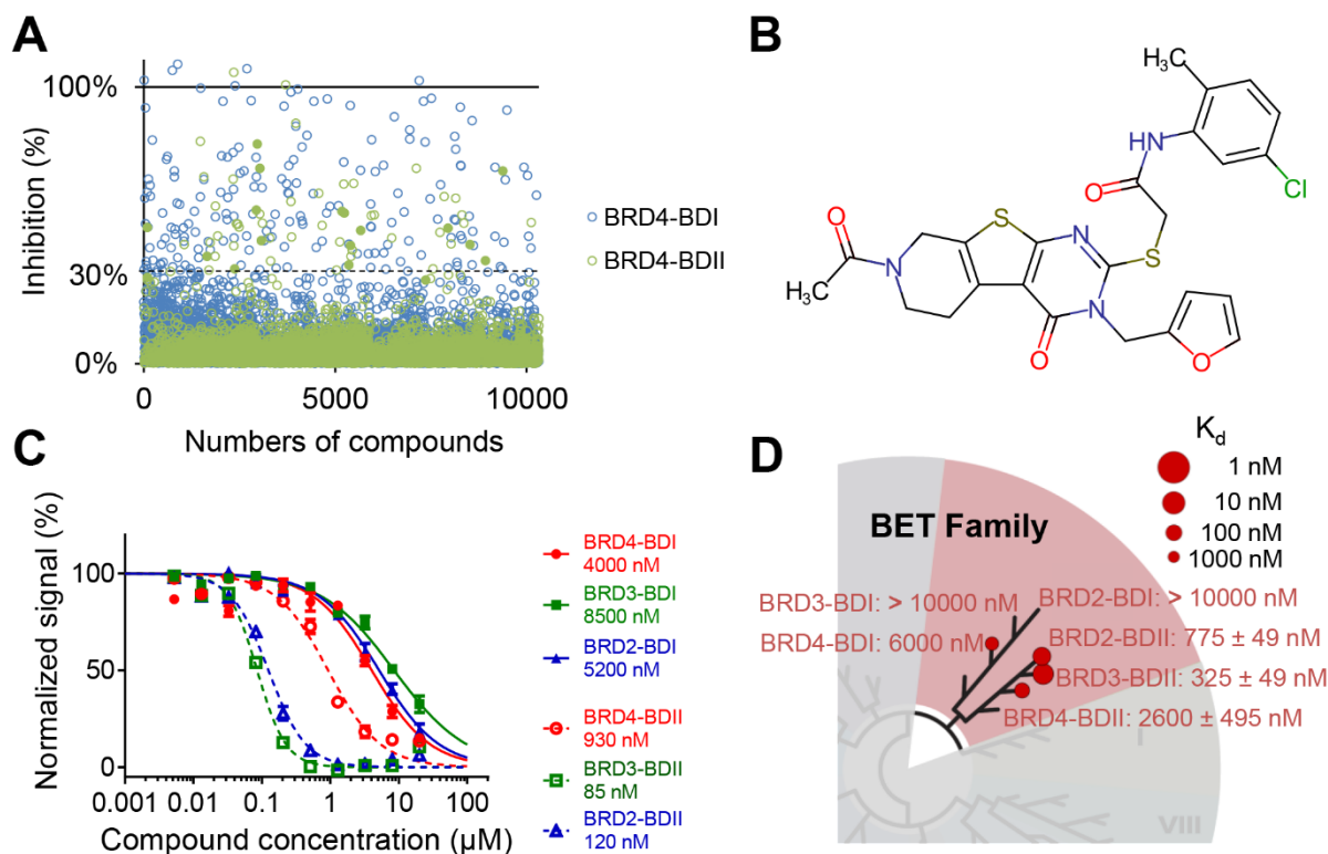
1 2 Figure 2. Fr-PPICChem screening and compound 1 characterization. (A) Scatter plot of Fr-PPICChem screening results against 3 BRD4-BDI (empty blue circles) and BRD4-BDII (empty green circles). BDII selective compounds identified above the 30% 4 threshold are shown as solid green circles. (B) Compound 1 chemical structure. (C) HTRF selectivity assay on the BDI (solid lines) 5 and BDII (dashed lines) of BRD2 (blue), BRD3 (green) and BRD4 (red). (D) BROMOscan data on the BET bromodomain family for 6 both BDs of BRD2, BRD3 and BRD4.
