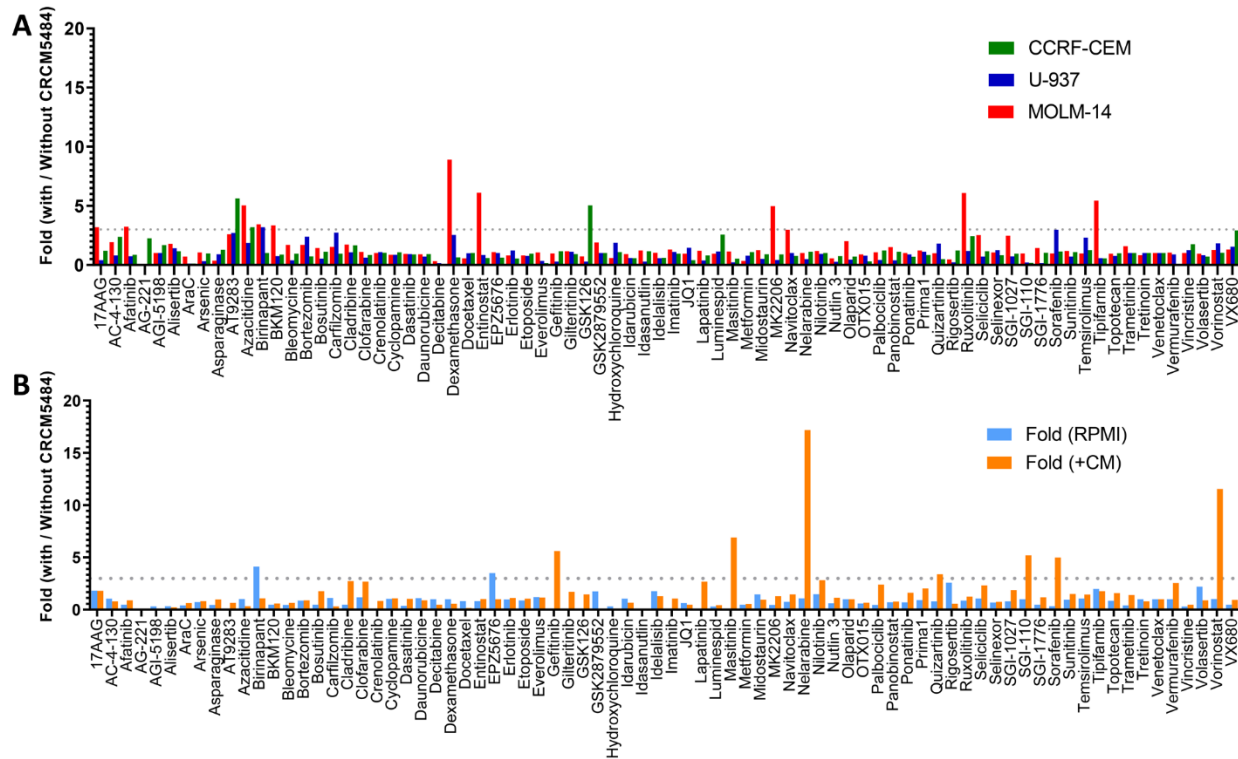
1 2 Figure 5. CRCM5484 potentiation of pharmacological agents. (A) Fold of drug cytotoxic effects with or without CRCM5484 at 3 its EC 40 (Table S2) in CCRF-CEM (green), U-937 (blue) and MOLM-14 (red) cell lines. (B) Fold of drug cytotoxic effects with or 4 without CRCM5484 with or without addition of bone-marrow-derived stromal cell conditioned medium (BMSC-CM).
