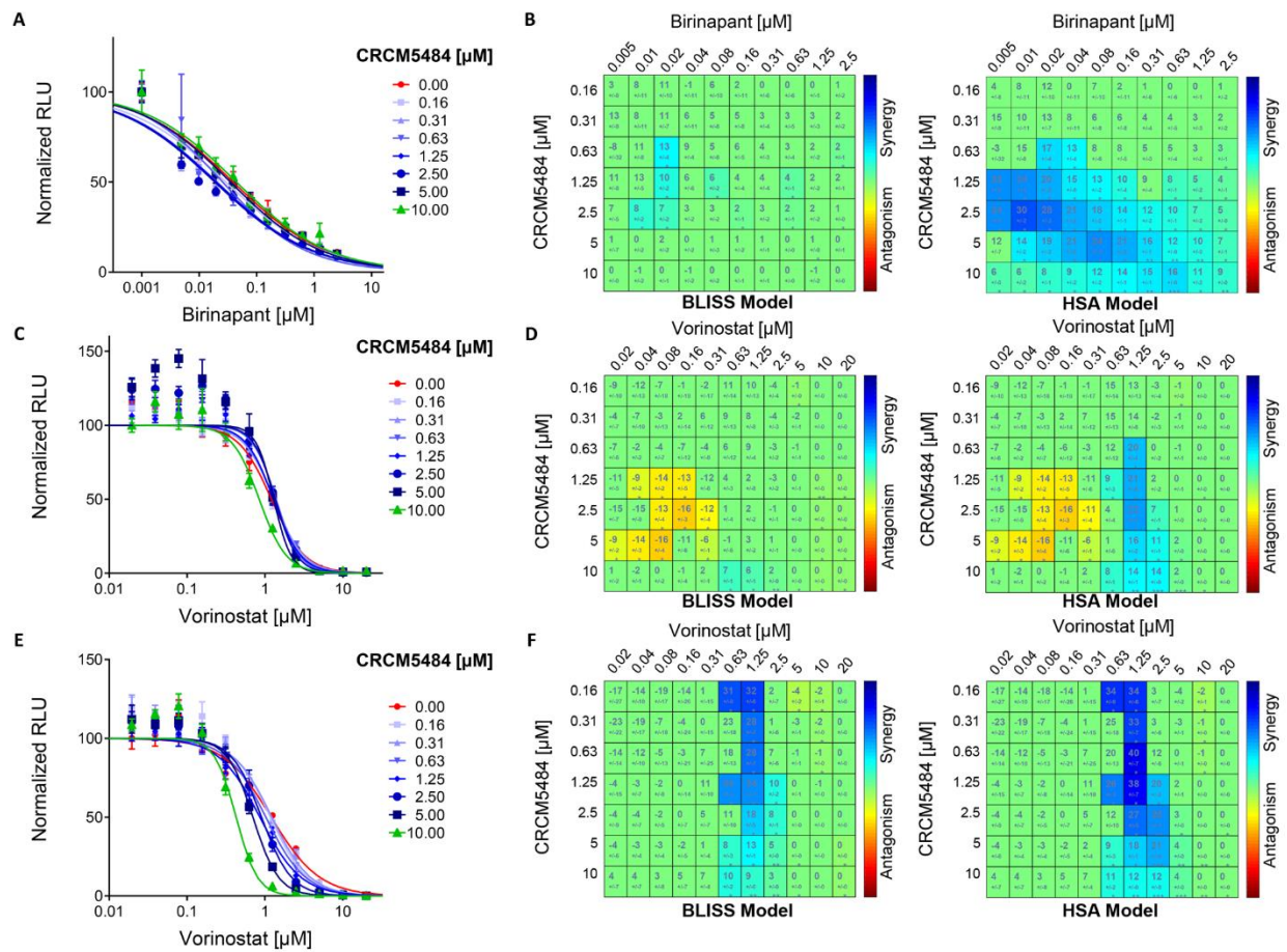
8 9 Figure 6. Validation of CRCM5484 potentiation of pharmacological agents in conditioned medium in the presence/absence of 10 BMSC-CM. Dose response curves of birinapant (A) or vorinostat (C and E) cytotoxic effect at a concentration range of 11 CRCM5484 in the absence (A and C) or the presence (E) of BMSC-CM. Combination effect matrix between birinapant (B) and 12 vorinostat (D and F) in combination with CRCM5484 analyzed using the BLISS (right) and HSA model (left) in the absence (B and 13 D) or the presence (F) of BMSC-CM. The synergy/antagonism score and its statistical significance is specified for each 14 combination. Significant combinations are colored in an antagonism/synergy scale (red to blue) and stars indicate the level of 15 significance.
