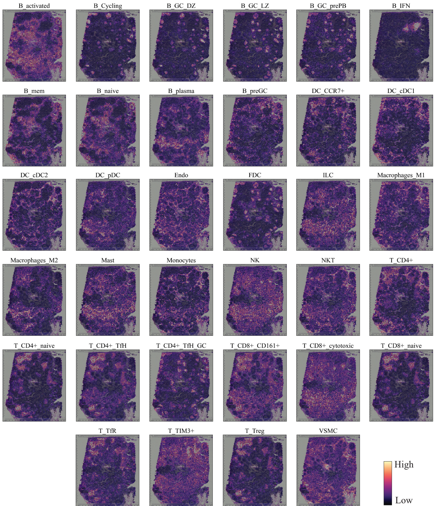
Figure S3. Spatial distributions predicted by cell2location of all 34 cell types in human lymph node dataset.
