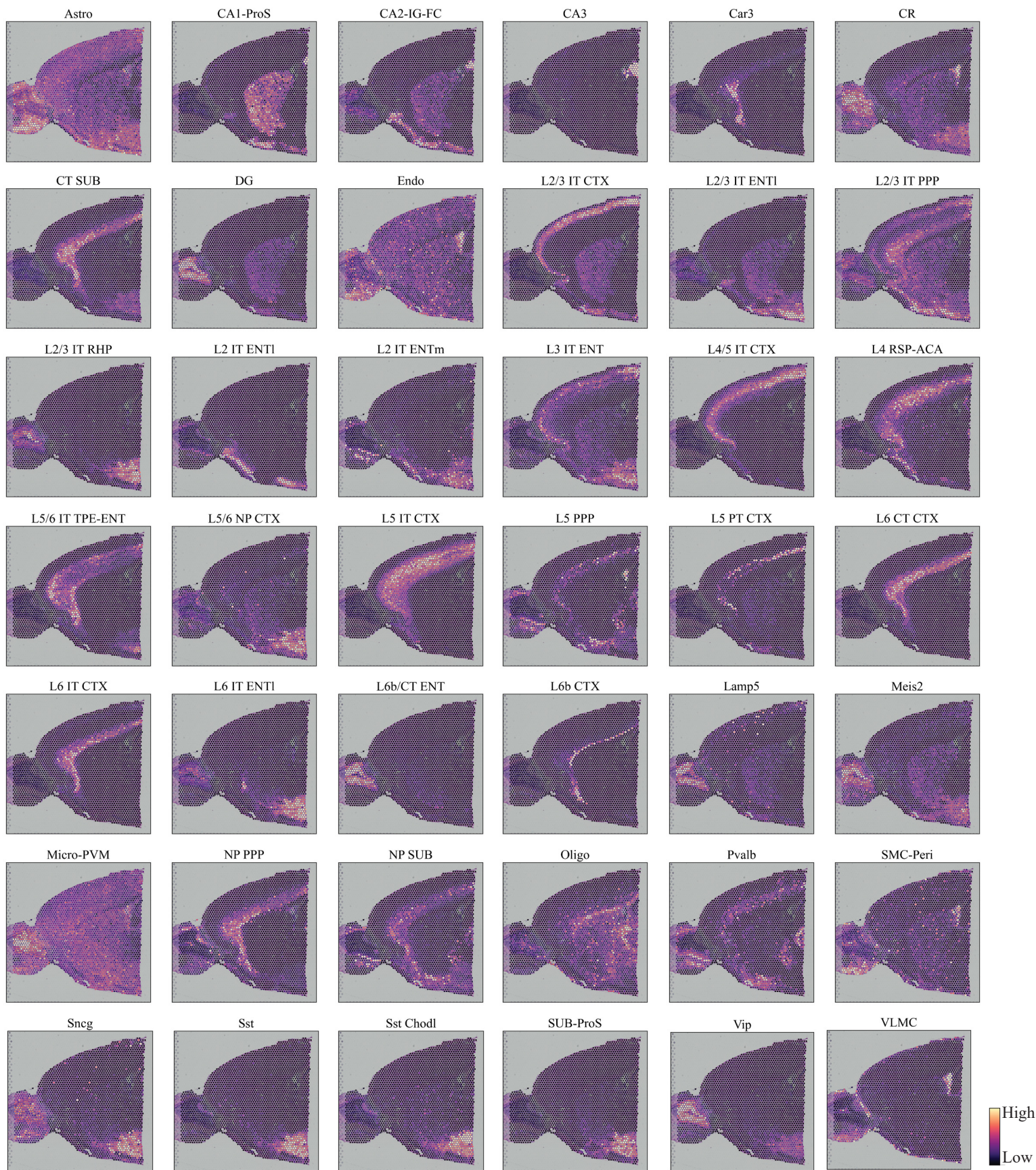
Figure S5. Spatial distributions predicted by cell2location of all 42 cell types in mouse brain anterior dataset.
