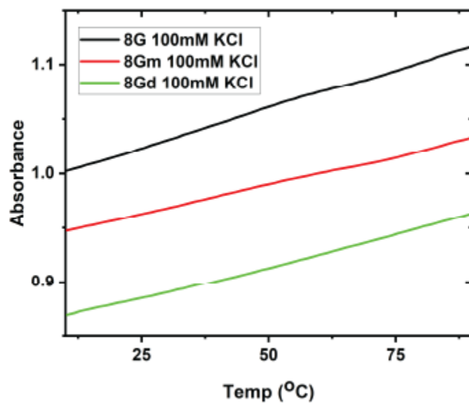
Figure S1. Thermal denaturation curves monitored by the change in absorbance at 260 nm.
