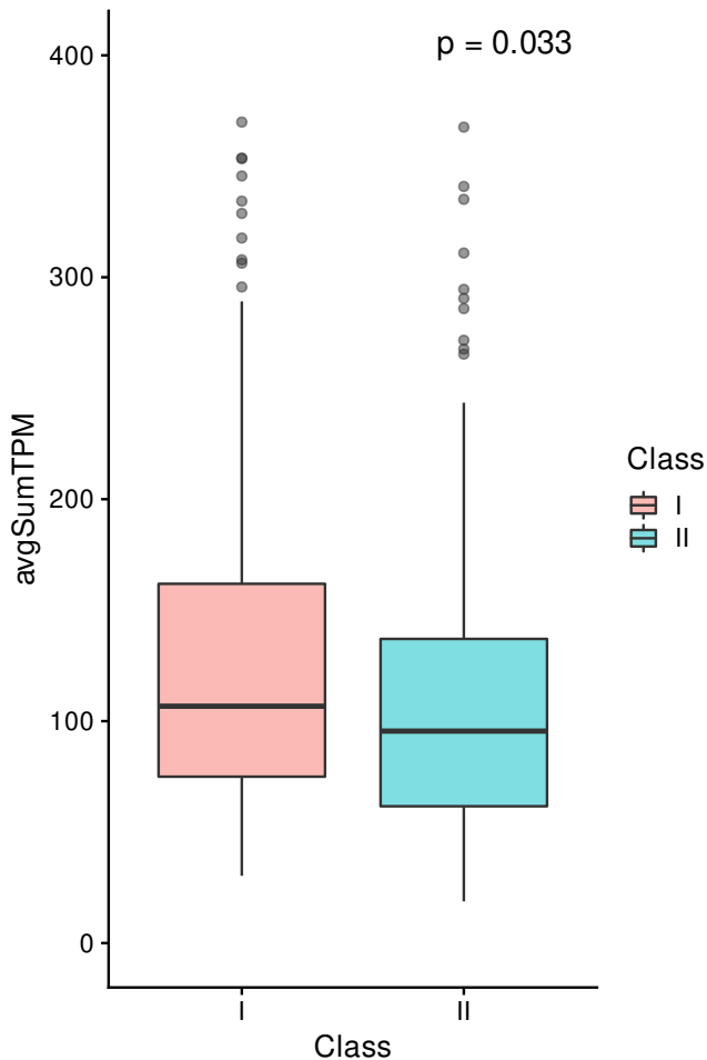
Fig S7. Comparison of average TPM of genes from Class I and II GO terms for homoeologous pairs that are affected by homoeologous exchange. P-value represents the results of a Kruskal-Wallis test
