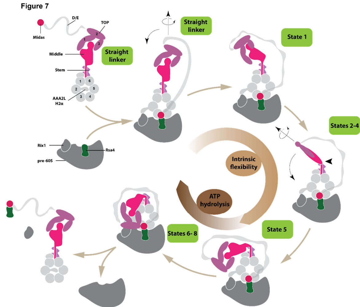
Figure 7: Model for the Rea1 mechanism. Rea1 in the absence of pre60S particles exists in an autoinhibited form with the AAA2H2 \alpha insert occupying the central pore of the AAA+ ring and the linker in the straight conformation. The binding of Rea1 to pre60S particles relocates AAA2H2 \alpha towards the pre60S particles which allows the MIDAS domain to dock onto the AAA+ ring to engage with its assembly factor substrate (here Rsa4). The linker remains in the straight conformation. The linker subsequently rotates and pivots towards the plane of the AAA+ ring to reach state 1. From here the linker middle and top domains rotate around the long linker axis and swing towards the AAA+ ring. The region between the linker middle and stem domains acts as pivot point. In state 5, the linker middle and top domains are fully rotated and in close proximity to the AAA+ ring. In states 6-8, the linker top engages with the AAA+ ring and in the final remodelling step state 8 the linker top2 domain interacts with the MIDAS domain to allow the transmission of force for assembly factor removal. Up to state, the linker remodelling is nucleotide independent and driven by the intrinsic conformational flexibility of the linker. States 6 – 8 require ATP hydrolysis.
