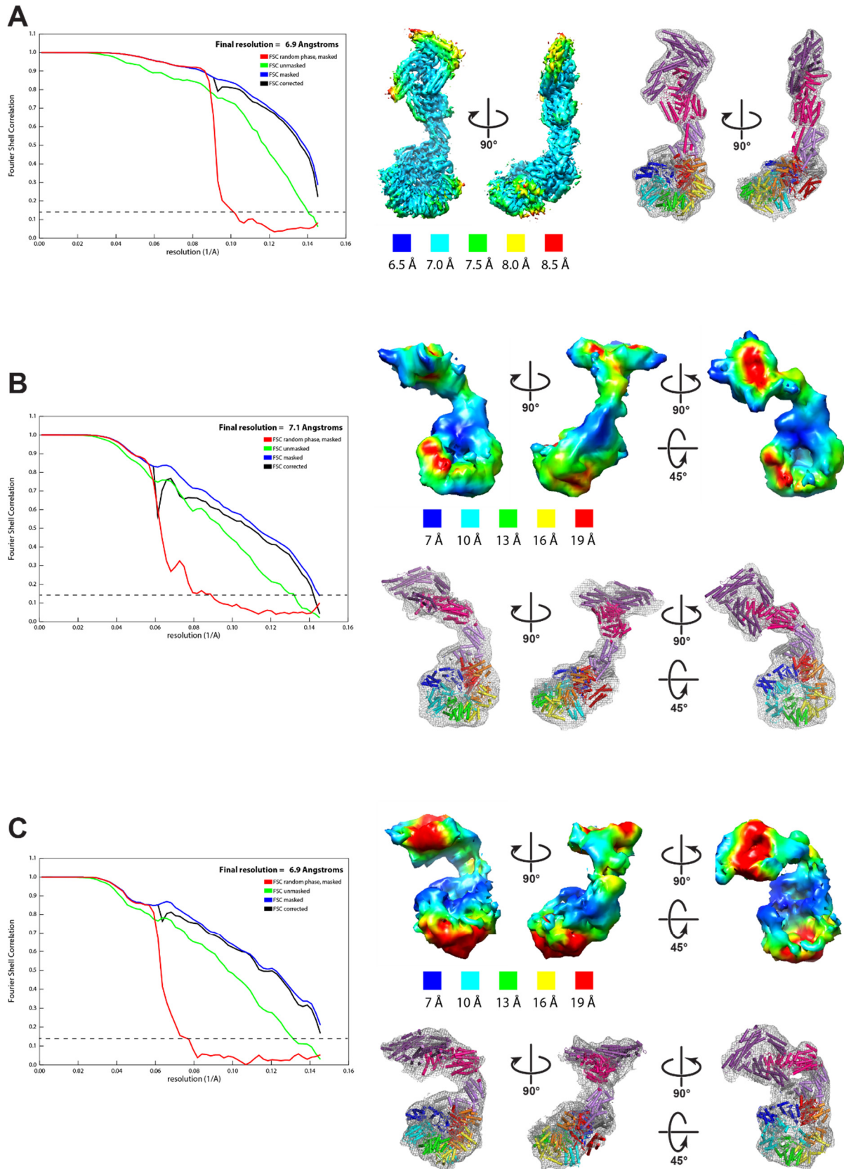
Supplementary figure 10: Overall quality of the Rea1 D2915A-R2976A-D3042A ATP cryoEM maps. Fourier shell correlation (FSC) plot for half-maps of the 3D reconstructions (left panels, 0.143 FSC criteria is indicated as horizontal dashed line), local resolution maps (middle and right panels) and match of structure in map (right and lower right panels) of A . Conformation I, B . Conformation II and C . Conformation III. In
