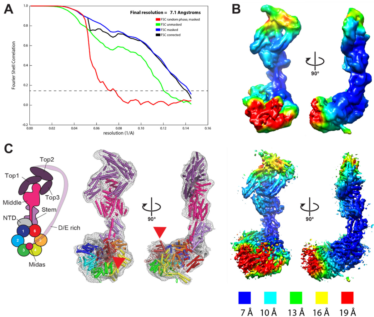
Supplementary figure 3: Overall quality of the Rea1 \Delta AAA2H2 \alpha ATP \gamma S cryoEM map. A. Fourier shell correlation (FSC) plot for half-maps of the 3D reconstruction. The 0.143 FSC criteria is indicated as horizontal dashed line. The final overall resolution is 7.1 Å. B. Local resolution map, upper panels: unsharpened map, lower panels: B-factor sharpened map. Secondary structure elements can be identified. C. Schematic cartoon representation of structure (left) and match of structure in map (right). Red arrow heads highlight the AAA+ ring docked MIDAS domain.
