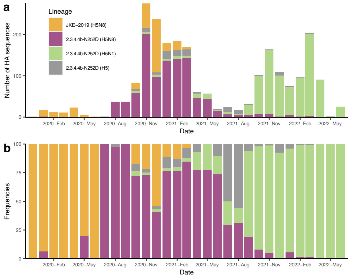
Supplementary fig. 3. Temporal changes in HPAI H5 lineage predominance. (a) The number of HA sequences colored by lineage since 2020. (b) Proportional lineage distribution by month inferred from (a).
