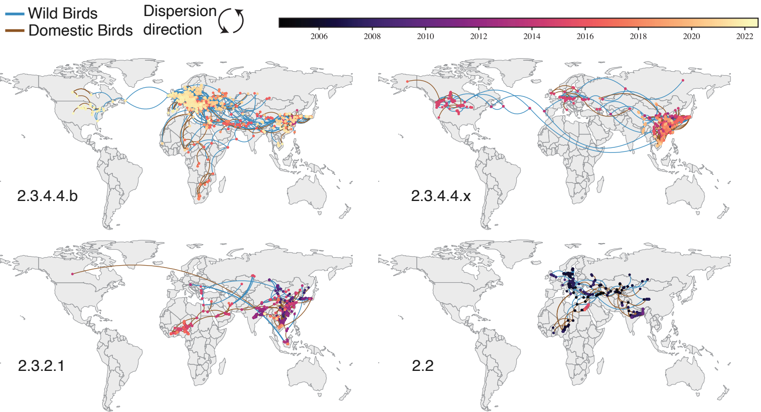
Supplementary fig. 5. Dynamics of HPAI H5 transmission lineages in clades 2.3.4.4.b, 2.3.4.4.x, 2.3.2.1 and 2.2. Virus lineage movements inferred by continuous phylogeographic analysis for each clade.
