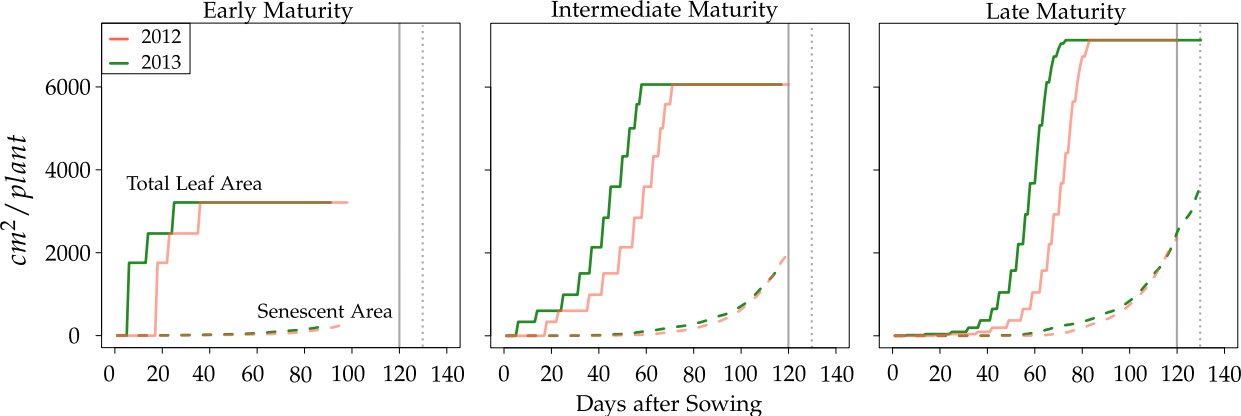
Figure S1. Simulated development of total and senescent leaf area. The early, intermediate and late maturing genotypes had a total leaf number (TLN) of 6, 14.5 and 23, respectively. The values for the other three traits were 750 for AM, 1.6 for SRE and 1150 for MTU and in common for all genotypes. The full and dotted vertical lines indicate the end of the 2012 and 2013 growing season, respectively.
