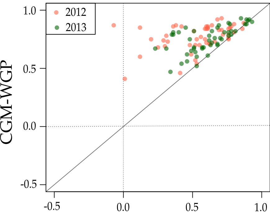
Observed Environments
