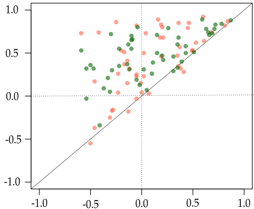
New Environments
