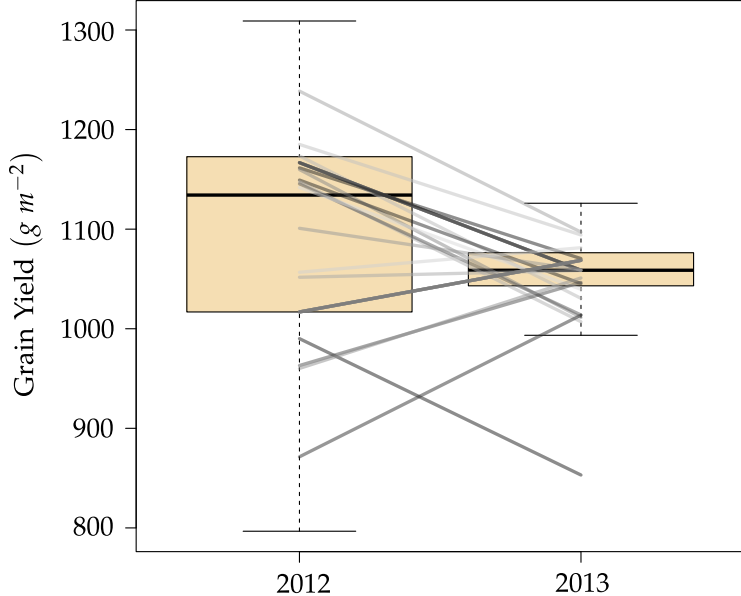
Figure S3. Distribution of simulated grain yield in 2012 and 2013 environments. The grey lines indicate the performance of specific genotypes in both environments. Data shown is from a representative example replication.
