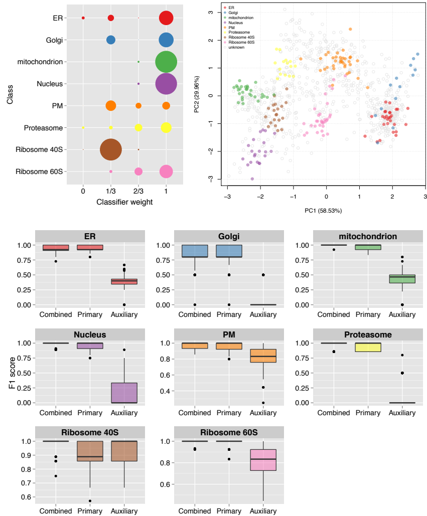
S1 File. Figure 4. k -NN transfer learning results for the fly dataset Top left: Bubble plot, displaying the distribution of the optimised class weights over the 100 test partitions for the transfer learning algorithm applied to the plant callus LOPIT and GO CC datasets. Top right: Principal components analysis plot of the LOPIT data (first and second components, of the possible four), showing the clustering of proteins according to their density gradient distributions. Bottom: Sub-cellular class-specific box plots, displaying the estimated generalisation performance over 100 test partitions for the transfer learning algorithm applied with (i) optimised class-specific weights (combined, both LOPIT and GO CC), (ii) only primary LOPIT data and (iii) only auxiliary GO CC data, for each sub-cellular class.
