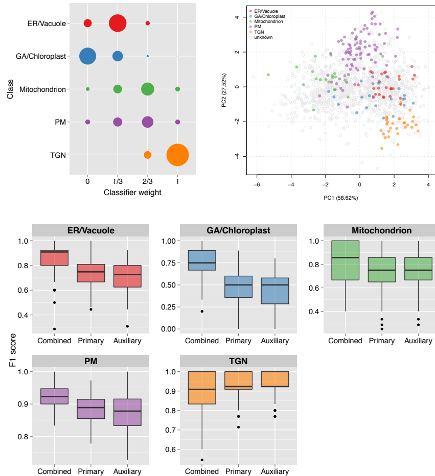
S1 File. Figure. 3. k -NN transfer learning results for the plant roots dataset Top left: Bubble plot, displaying the distribution of the optimised class weights over the 100 test partitions for the transfer learning algorithm applied to the plant callus LOPIT and GO CC datasets. Top right: Principal components analysis plot of the LOPIT data (first and second components, of the possible six), showing the clustering of proteins according to their density gradient distributions. Bottom: Sub-cellular class-specific box plots, displaying the estimated generalisation performance over 100 test partitions for the transfer learning algorithm applied with (i) optimised class-specific weights (combined, both LOPIT and GO CC), (ii) only primary LOPIT data and (iii) only auxiliary GO CC data, for each sub-cellular class.
