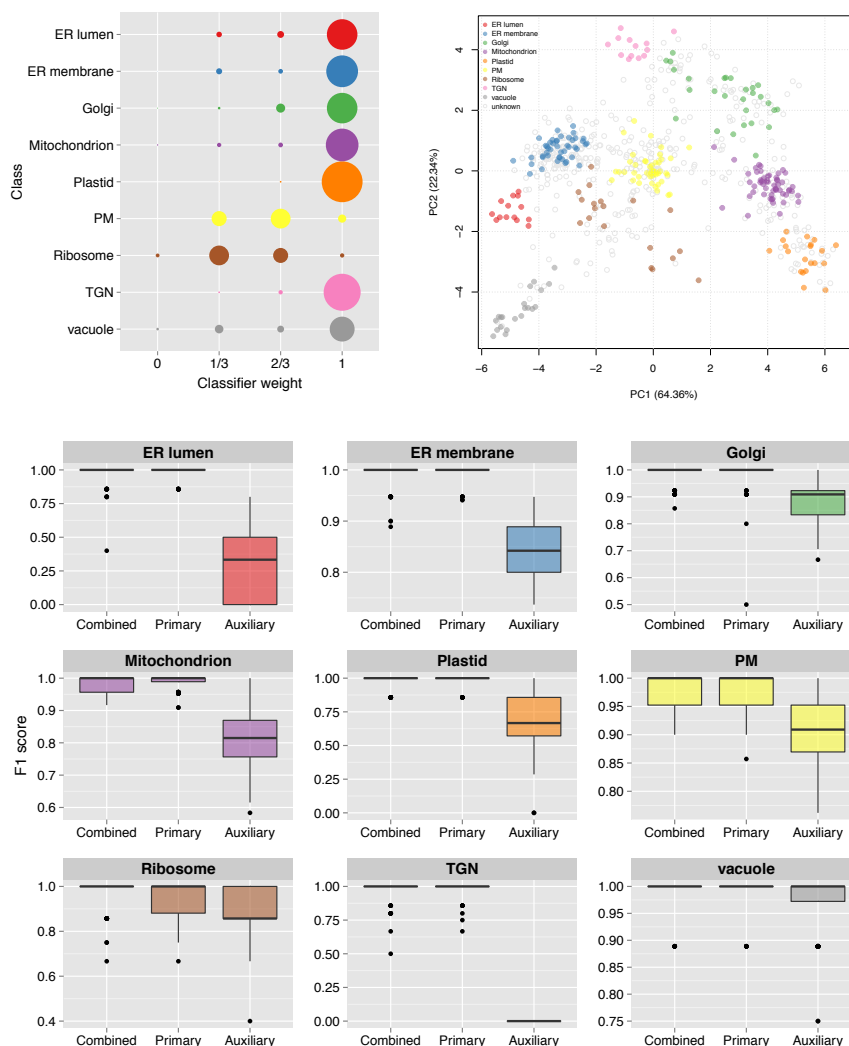
S1 File. Figure. 1. k -NN transfer learning results for the plant callus dataset Top left: Bubble plot, displaying the distribution of the optimised class weights over the 100 test partitions for the transfer learning algorithm applied to the plant callus LOPIT and GO CC datasets. Top right: Principal components analysis plot of the LOPIT data (first and second components, of the possible sixteen), showing the clustering of proteins according to their density gradient distributions. Bottom: Sub-cellular class-specific box plots, displaying the estimated generalisation performance over 100 test partitions for the transfer learning algorithm applied with (i) optimised class-specific weights (combined, both LOPIT and GO CC), (ii) only primary LOPIT data and (iii) only auxiliary GO CC data, for each sub-cellular class.
