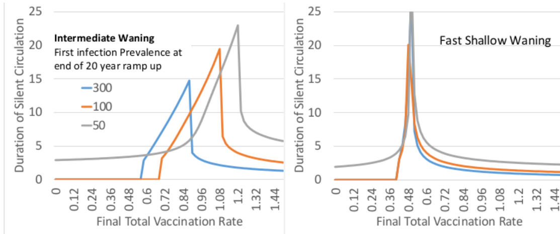
Figure 8: Silent circulation duration as a function of final total vaccination levels across values the endpoint prevalence of first infection from 300 to 50. Settings are for the intermediate and fast shallow waning scenario, a 20 year ramp-up time, and poliovirus type 3 infection to paralysis ratios and intermediate transmissibility of vaccine.
