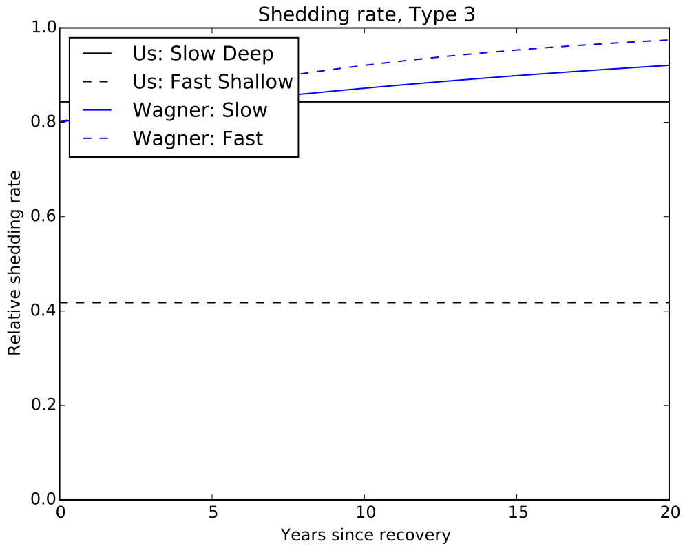
Figure 6: Curves showing relative intensity of virus shedding while infected with Type 3 poliovirus (compared to an immunologically naive individual) vs. time since previous Type 3 infection in years, under different models of immune waning. Curves for our model are shown in black, and curves for the Wagner et al. model in blue. For each model, the solid line represents the sub-model with slowest waning, while the dashed line represents the sub-model with the fastest waning. The curve for our “intermediate” model is not shown. The curves for the Wagner et al. model reflect relative risk of infection following a challenge dose of 10^{5.8} TCID 50 of OPV3; the curves for our model are the same regardless of challenge dose, for reasons discussed in the text.
