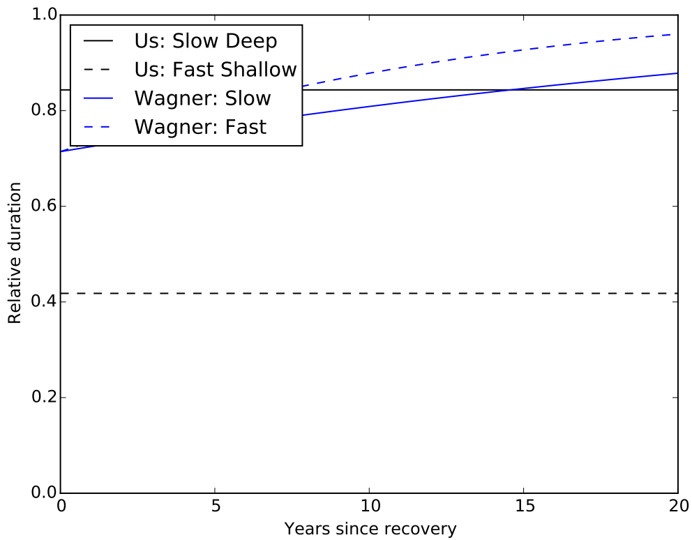
Figure 5: Curves showing relative average duration of infection while infected with Type 3 poliovirus (compared to an immunologically naive individual) vs. time since previous Type 3 infection in years, under different models of immune waning. Curves for our model are shown in black, and curves for the Wagner et al. model in blue. For each model, the solid line represents the sub-model with slowest waning, while the dashed line represents the sub-model with the fastest waning. The curve for our “intermediate” model is not shown. The curves for the Wagner et al. model reflect relative risk of infection following a challenge dose of 10^{5.8} TCID 50 of OPV3; the curves for our model are the same regardless of challenge dose, for reasons discussed in the text.
