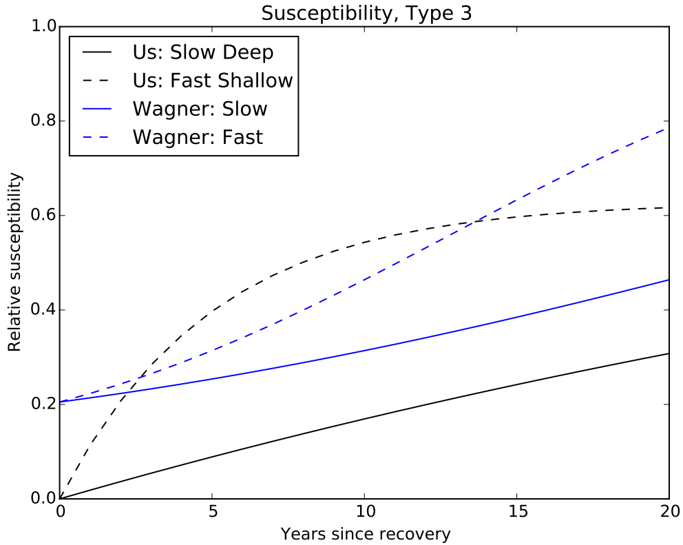
Figure 4: Curves showing relative risk of infection with Type 3 poliovirus (compared to an immunologically naive individual) vs. time since previous Type 3 infection in years, under different models of immune waning. Curves for our model are shown in black, and curves for the Wagner et al. model in blue. For each model, the solid line represents the sub-model with slowest waning, while the dashed line represents the sub-model with the fastest waning. The curve for our “intermediate” model is not shown. The curves for the Wagner et al. model reflect relative risk of infection following a challenge dose of 10^{5.8} TCID 50 of OPV3; the curves for our model indicate relative risk of infection following a cumulative exposure that would produce the same probability of infection in an immunologically naive individual as 10^{5.8} TCID 50 of OPV3 would produce in the Wagner model.
