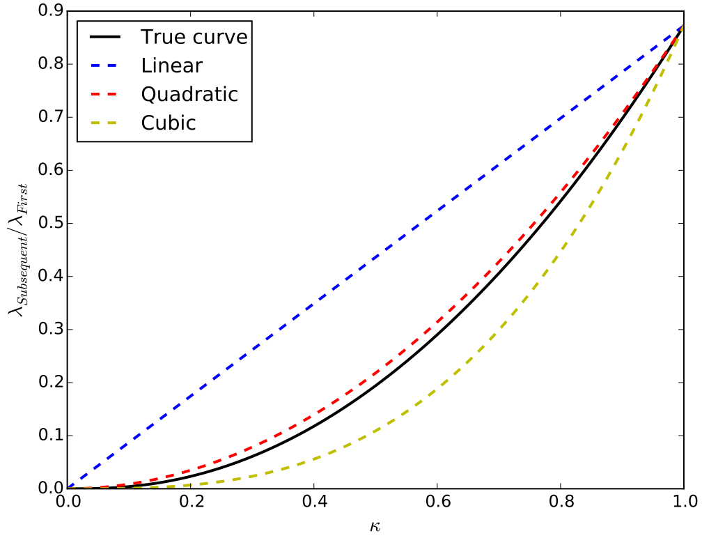
Figure 3: Dependence of \frac{\lambda_{\text{Subsequent}}}{\lambda_{\text{First}}} on \kappa . All parameters other than \kappa are set to the values they have in the “slow deep” scenario for the high transmission setting in the main text. For comparison, linear, quadratic, and cubic curves having the same two endpoints are shown as dashed lines.
