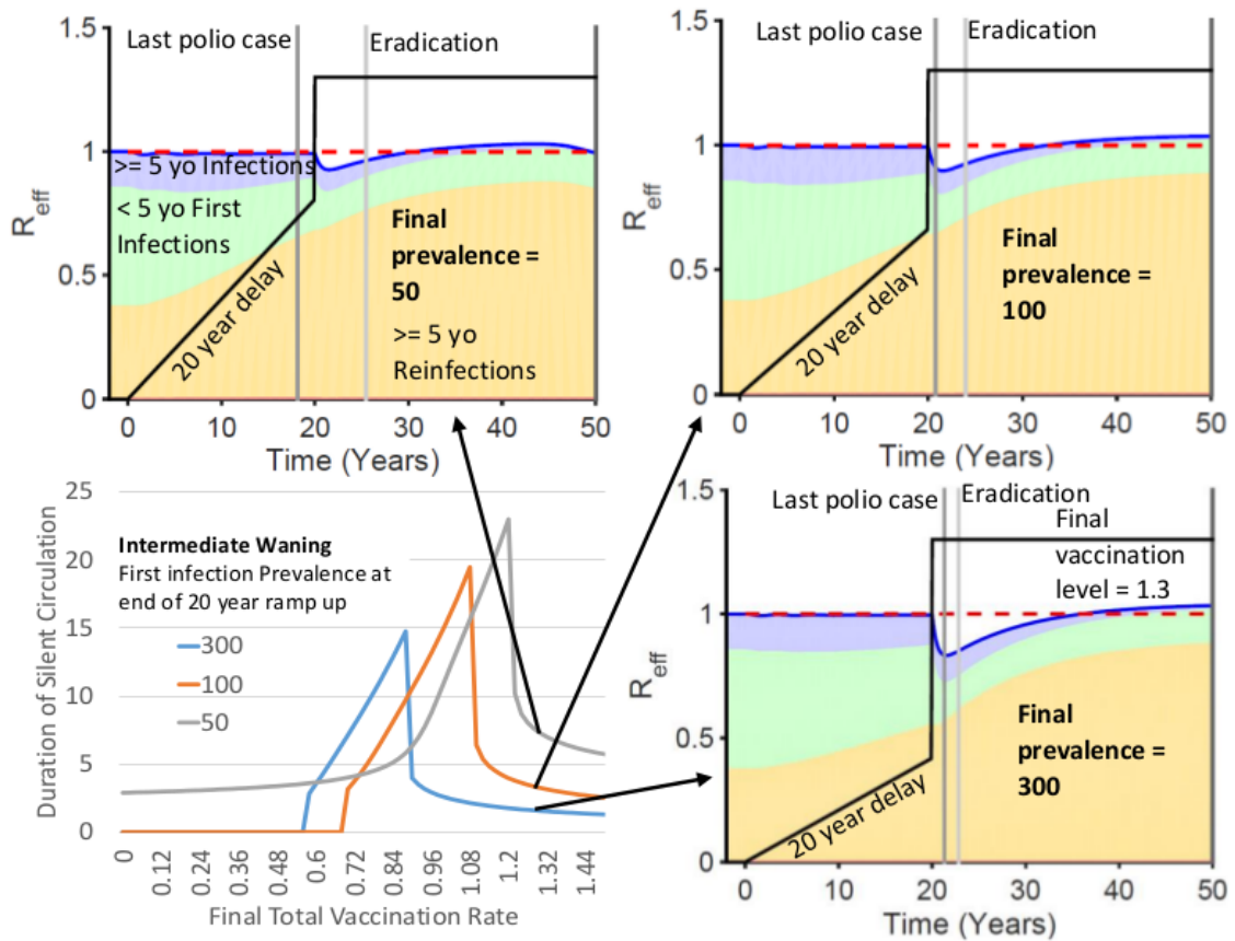
Figure 9: Comparison of effective reproduction number dynamics as the first infection prevalence at the end of a 20 year ramp up becomes increasingly lower for intermediate waning.
