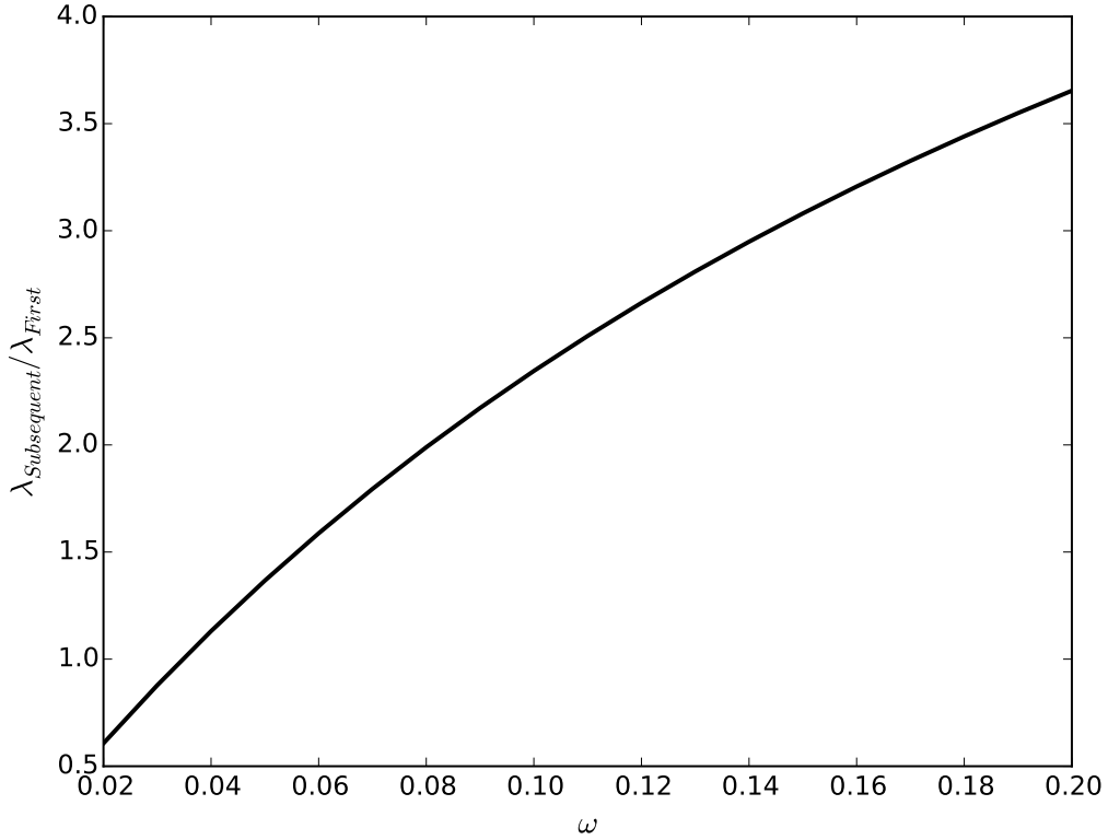
Figure 2: Dependence of \frac{\lambda_{\text{Subsequent}}}{\lambda_{\text{First}}} on \omega . All parameters other than \omega are set to the values they have in the “slow deep” scenario for the high transmission setting in the main text.
