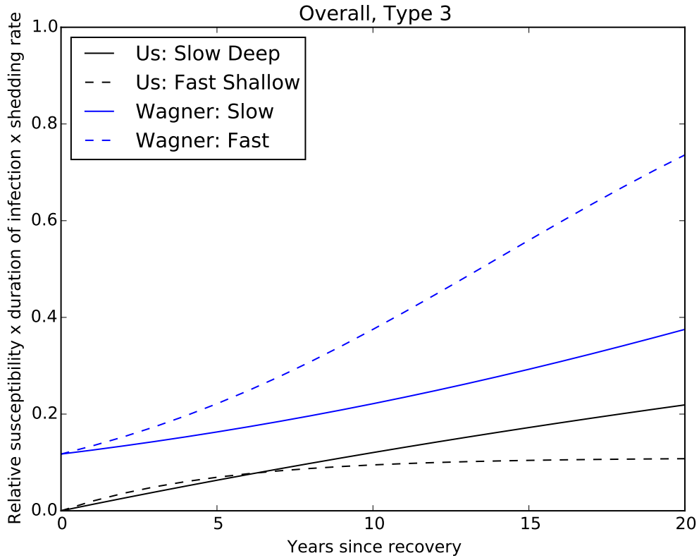
Figure 7: Curves showing relative probability of infection with Type 3 poliovirus times relative average duration of infection times relative shedding rate (compared to an immunologically naive individual) vs. time since previous Type 3 infection in years, under different models of immune waning. For our model, this is equivalent to the “population extent of waning” shown in Figure 2 in the main text. Curves for our model are shown in black, and curves for the Wagner et al. model in blue. For each model, the solid line represents the sub-model with slowest waning, while the dashed line represents the sub-model with the fastest waning. The curve for our “intermediate” model is not shown. The curves for the Wagner et al. model reflect relative risk of infection following a challenge dose of 10^{5.8} TCID 50 of OPV3; the curves for our model are the same regardless of challenge dose, for reasons discussed in the text.
