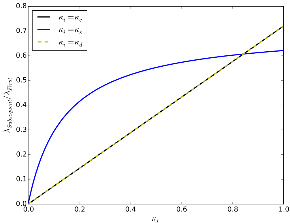
Figure 1: Dependence of \frac{\lambda_{\text{Subsequent}}}{\lambda_{\text{First}}} on \kappa_c , \kappa_s , and \kappa_d . In each curve, all parameters other than the \kappa_i being varied are set to the values they have in the “slow deep” scenario for the high transmission setting in the main text; in particular, both of the other two \kappa_j are fixed at 0.6^{1/3} .
