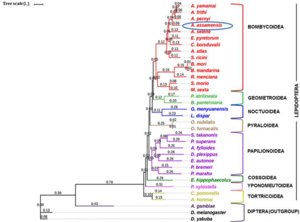
Figure S6. Molecular phylogeny inferred from whole mitogenome sequences of 34 organisms using Maximum Likelihood method. The scale for genetic distance is shown at the top of the figure and the numbers denote branch lengths of the tree.
