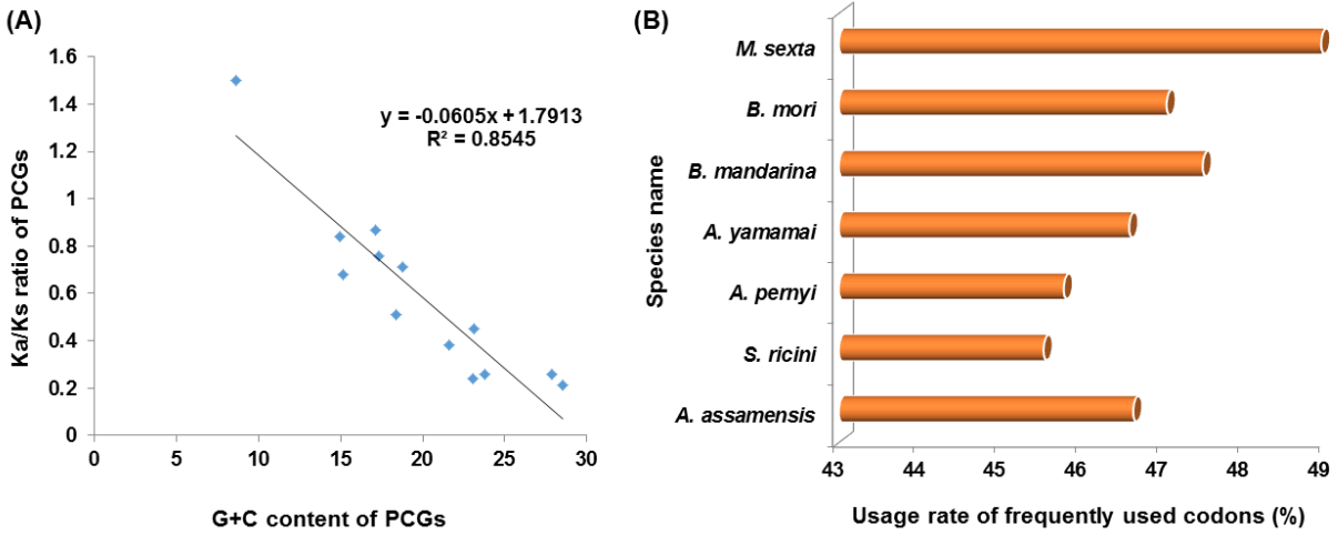
Figure S2. (A) G+C content versus Ka/Ks ratios of 13 concatenated PCGs in A. assamensis mitogenome (B) The usage rate of five frequently used codons in Bombycoidea members.
