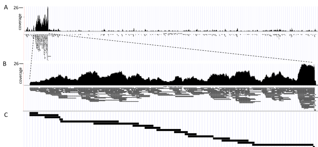
Figure S1. Nanopore sequencing coverage analysis of the 200 kbp target region. A. Coverage analysis (top) and read alignment (bottom) of the longest 10% reads to the entire E. coli genome. B. Coverage analysis (top) and read alignment (bottom) of the longest 10% reads to
