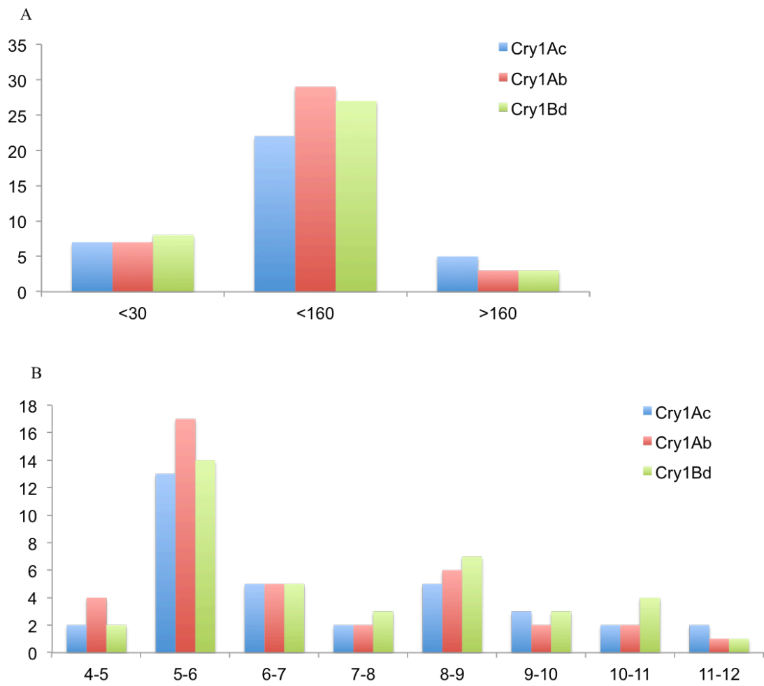
Supplemental Fig 2. Molecular range (A) and pH (B) of proteins detected from Cr1Ac, Cry1Ab, and Cry1Bd using the modified far-immunoblotting method.
