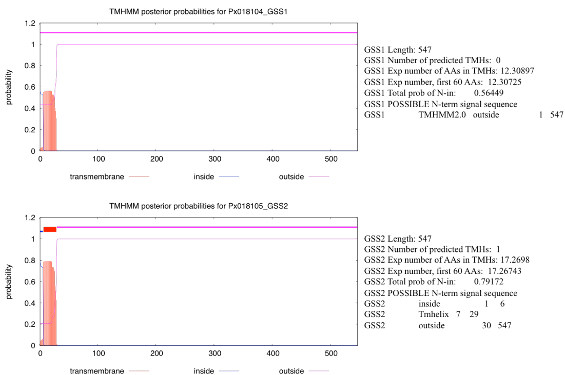
Supplemental Fig 4. Transmembrane helices of GSS1 (top) and GSS2 (bottom) analyzed by TMHMM.
