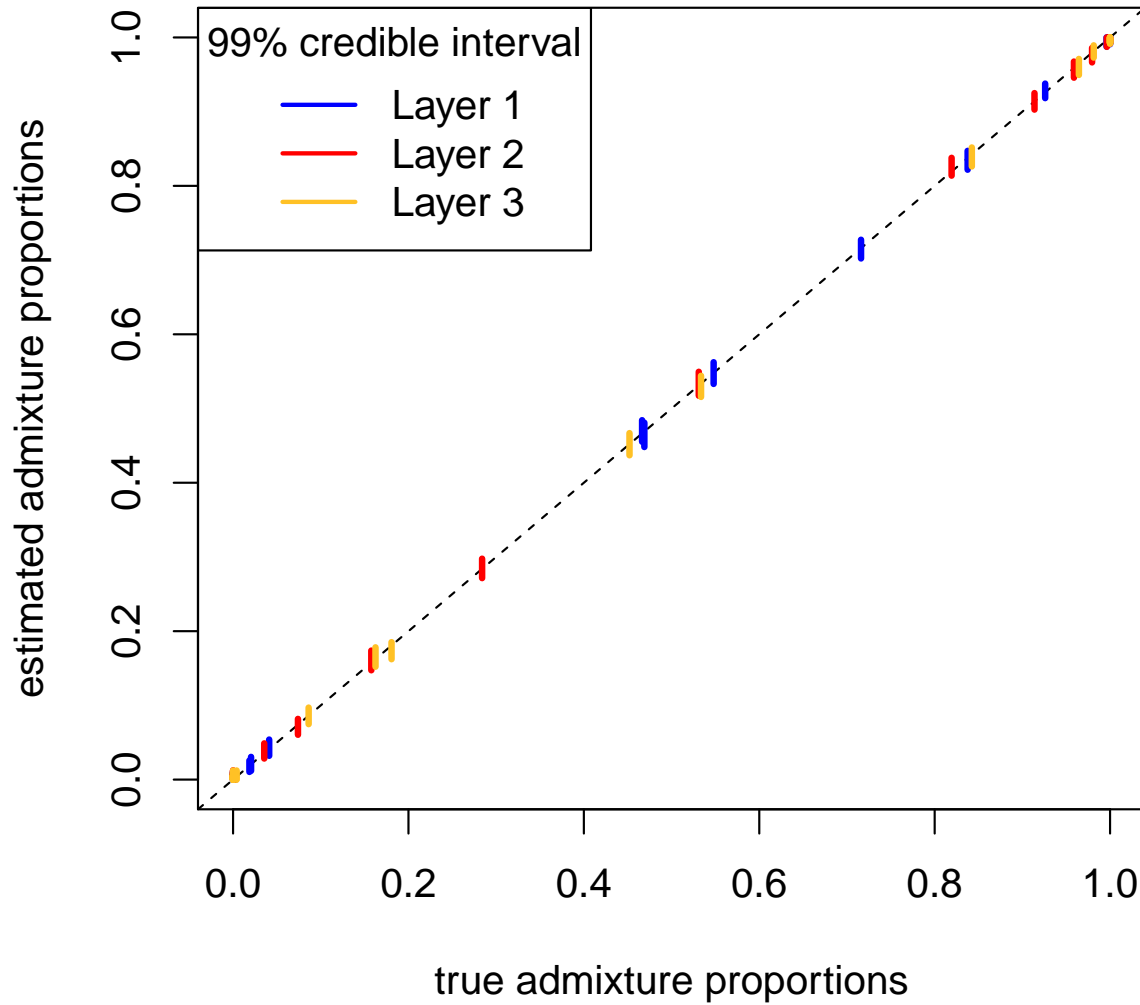
Fig S13. Plot of conStruct ability to correctly estimate admixture proportions on simulated data. Results are from an analysis with a spatial model using K = 3 .
