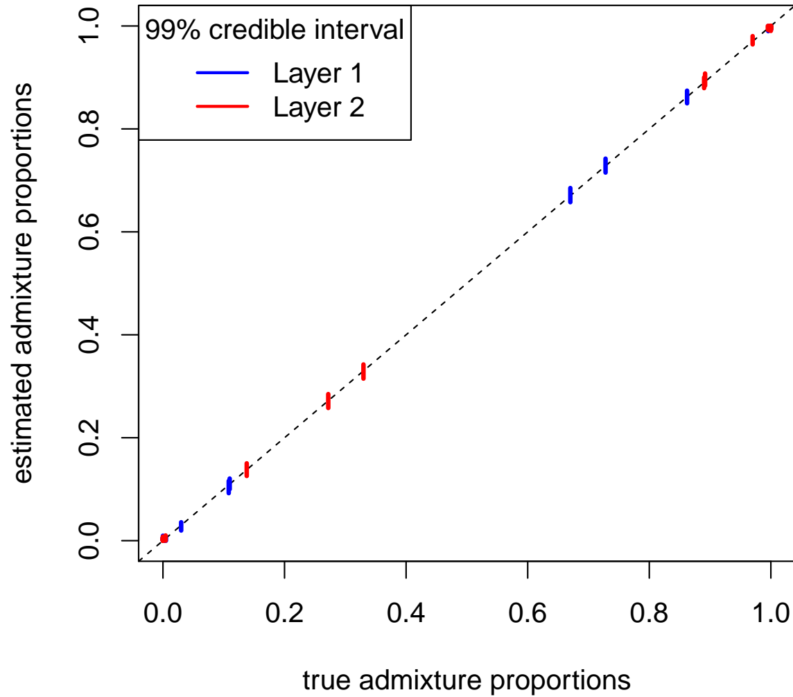
Fig S8. Plot of conStruct ability to correctly estimate admixture proportions on simulated data. Results are from an analysis with a spatial model using K = 2 .
