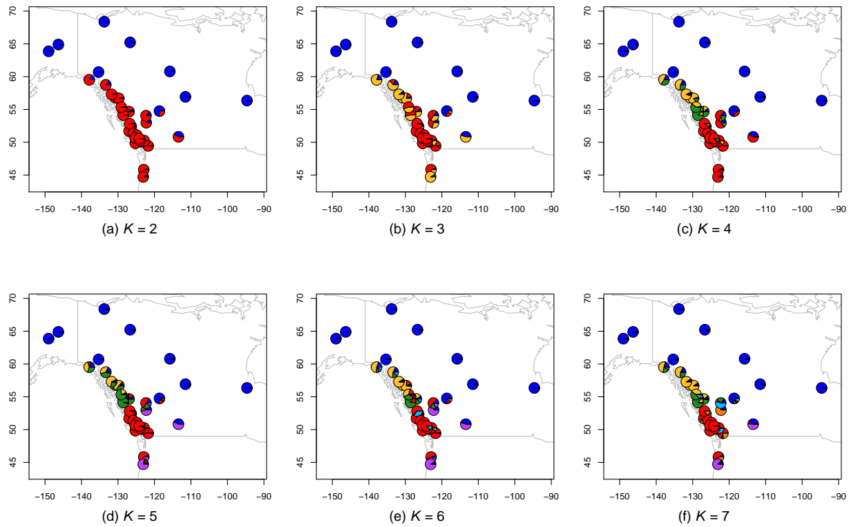
Fig S18. Maps of admixture proportions estimated for the Populus dataset using the spatial model for K = 2 through 7.
