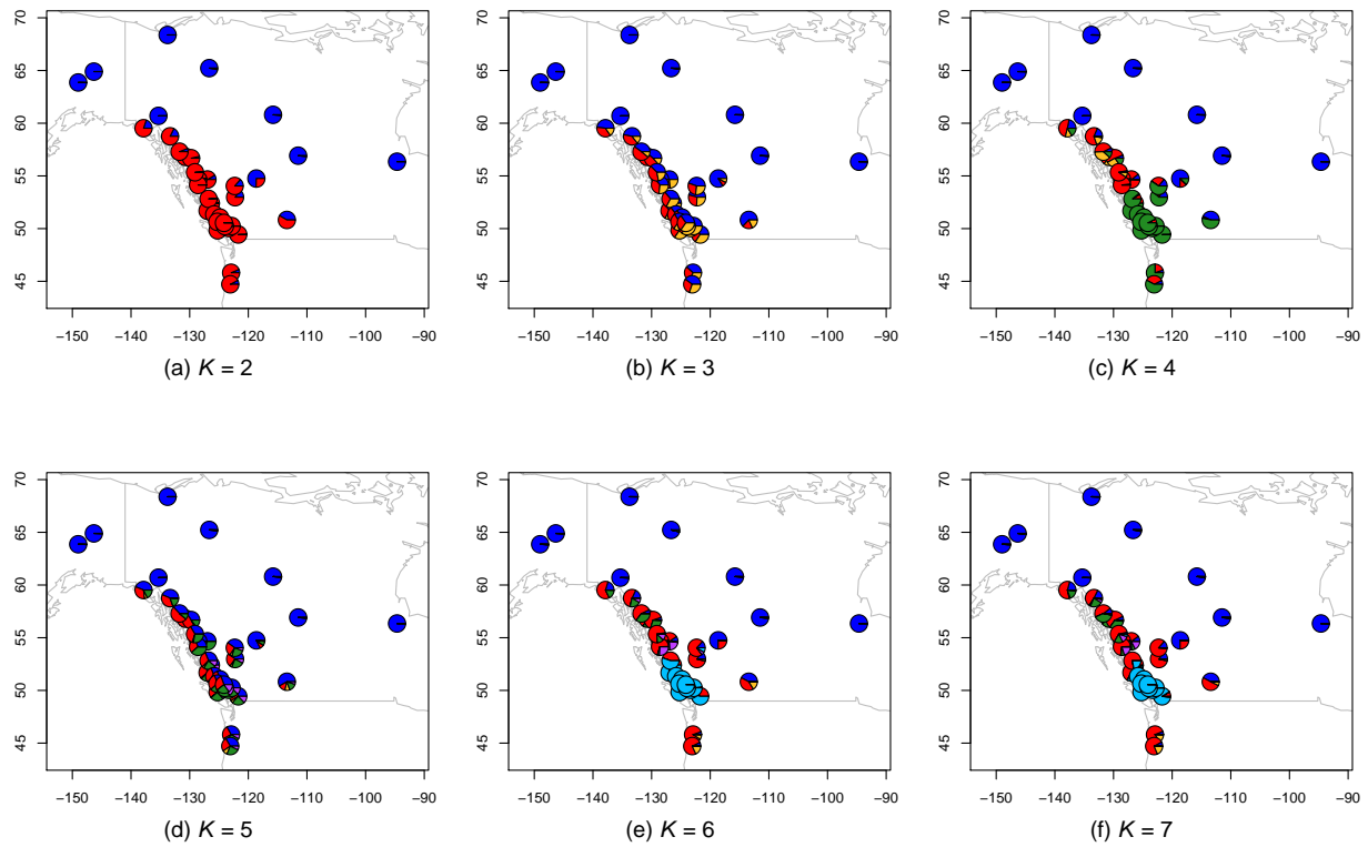
Fig S19. Maps of admixture proportions estimated for the Populus dataset using the nonspatial model for K = 2 through 7.
