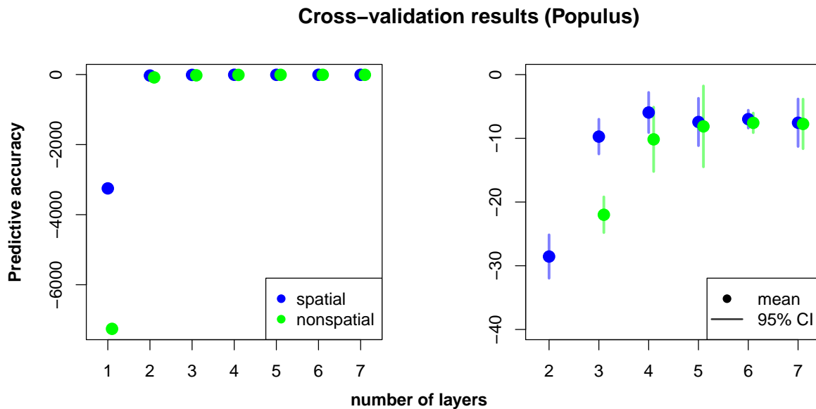
Fig 6. Cross-validation results for Populus dataset comparing the spatial and nonspatial conStruct models run with K = 1 through 7. The first panel in each row shows all results; the second panel zooms in on the results from analyses run with K = 2 through 7.
