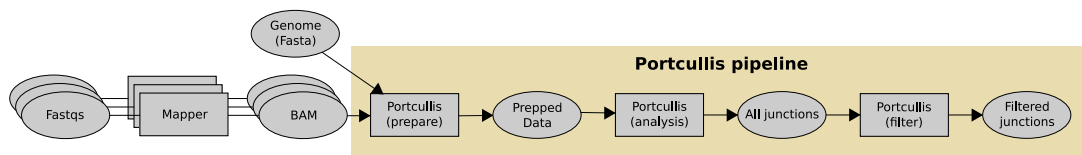
Fig. 8: A high level view of the Portcullis pipeline. Input to Portcullis is a genome in fasta format and one or more BAM files created by an upstream RNAseq mapping tool. The first stage ensures the alignments are correctly merged, sorted and indexed, then all junctions found in the input are analysed and output to disk. Next, the full set of junctions are filtered to remove likely false positives and are also output to disk. The user can either choose to run the full pipeline in one go, or each stage separately.
