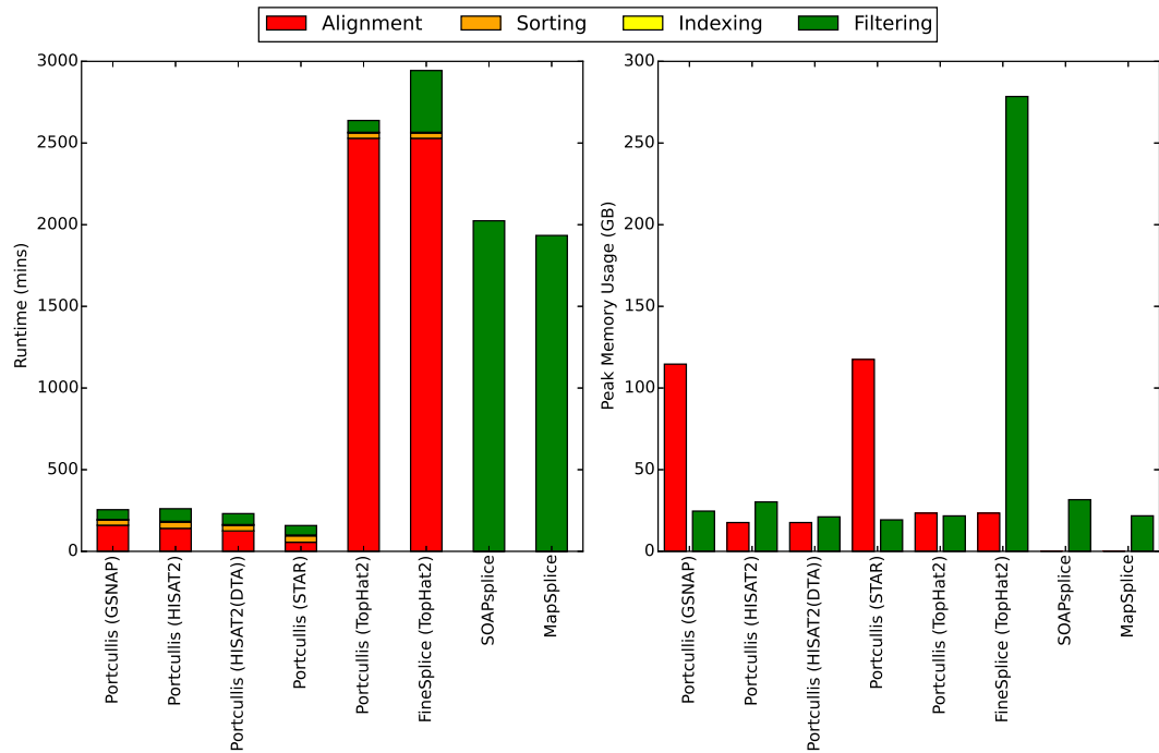
Fig. 5: Runtimes and max memory usage of all methods on our 101bp ~76 million simulated human read dataset using 8 threads where appropriate. For FINESplice and Portcullis, times for alignment, sorting and indexing are factored into the results. For memory usage we consider alignment and filtering stages only.
