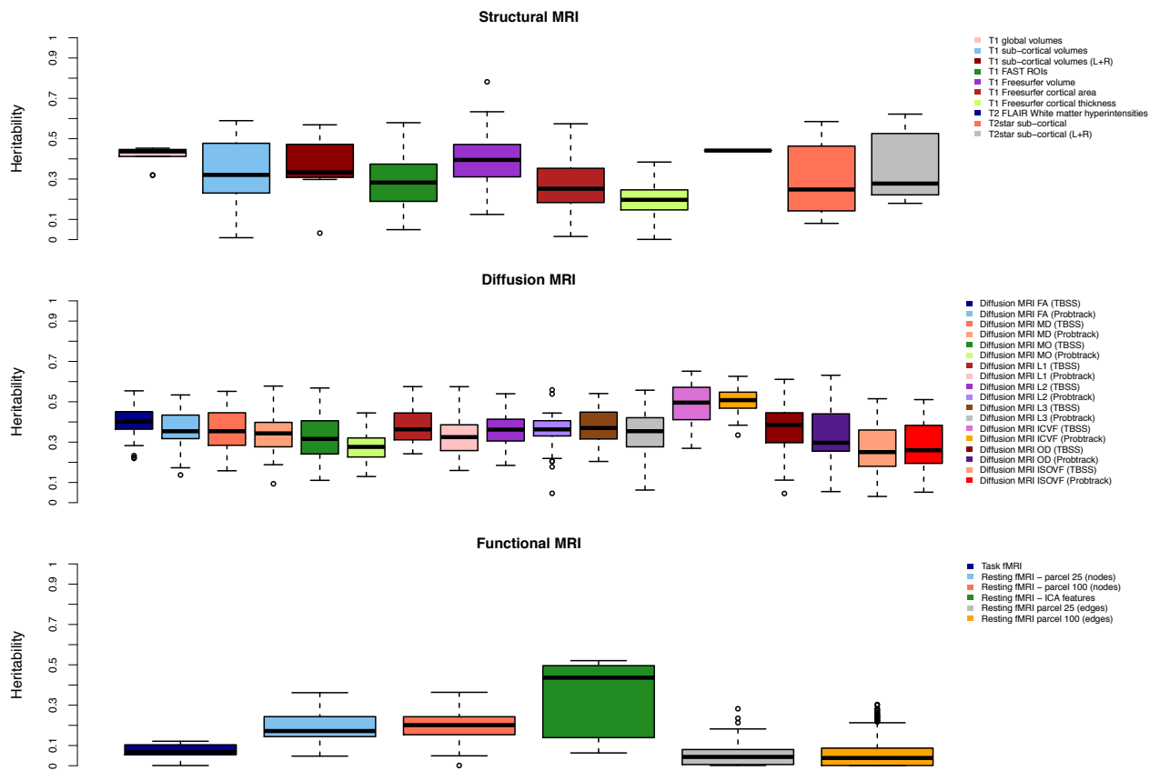
Supplementary Figure 1 : Estimated heritability of IDPs. Boxplots of estimated heritability (y-axis) for different IDP groups. IDPs have been split into three broad groups : Structural MRI (top), Diffusion MRI (middle) and Functional MRI (bottom). Boxplots are colored according to IDP groups.
