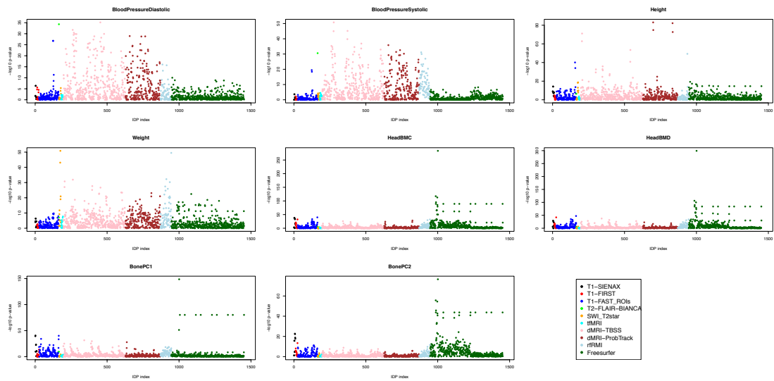
Supplementary Figure 21. Association of IDPs with Body Confounds. Each plot shows the association of a body confound measure with all of the IDPs except the resting fMRI parcellation edges.
