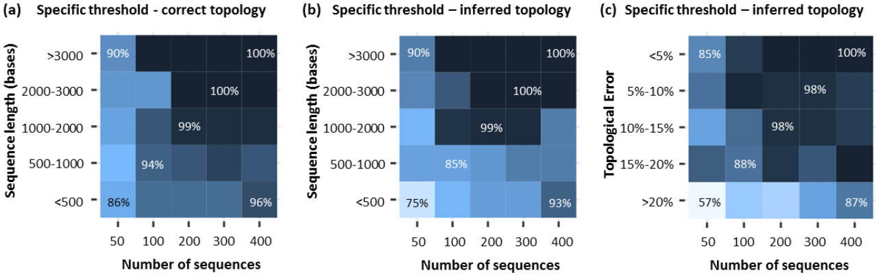
Figure S1. Patterns of CorrTest accuracy using M100, M200, M300, and M400 models for the corresponding test datasets (Tamura et al., 2012). Accuracies are shown for increasing number of sequences. The accuracy of CorrTest for different sequence length is shown when (a) the correct topology was assumed and (b) the topology was inferred. (c) The accuracy of CorrTest for datasets in which the inferred the topology contained small and large number of topological errors.
