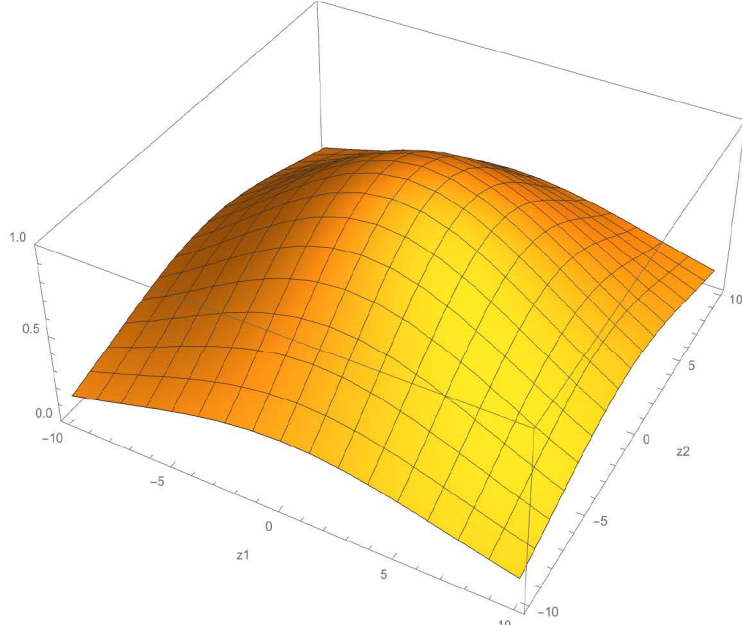
d \sigma^2 = 100
