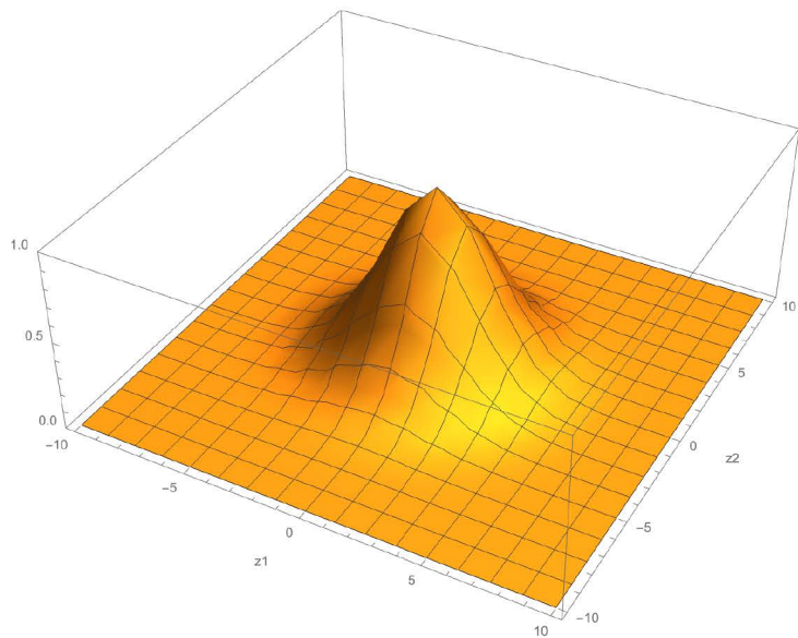
a \sigma^2 = 10
