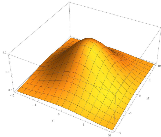
d \sigma^2 = 100
