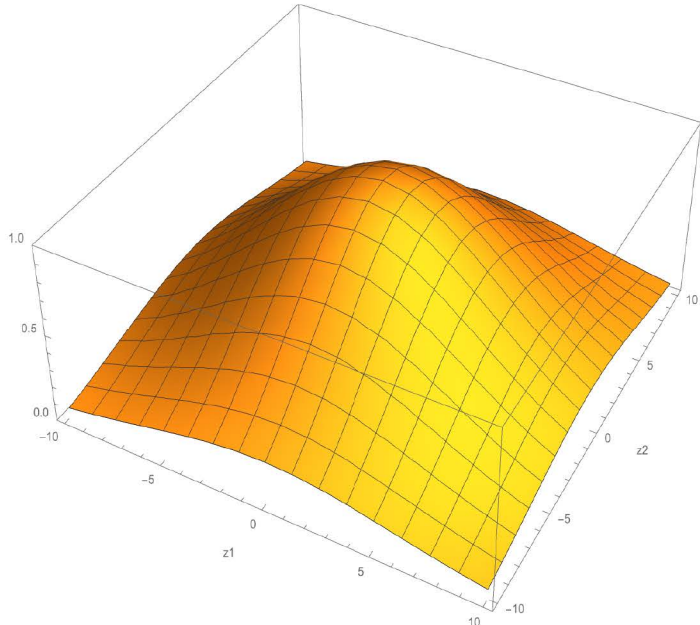
c \sigma^2 = 70
